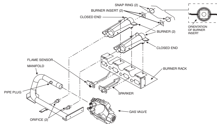
Fig. 7 - Two-Stage Orifice Installation
