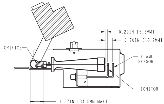
Fig. 4 - Two-Stage Igniter, Flame Sensor, Orifice/Main Burner Relationship
