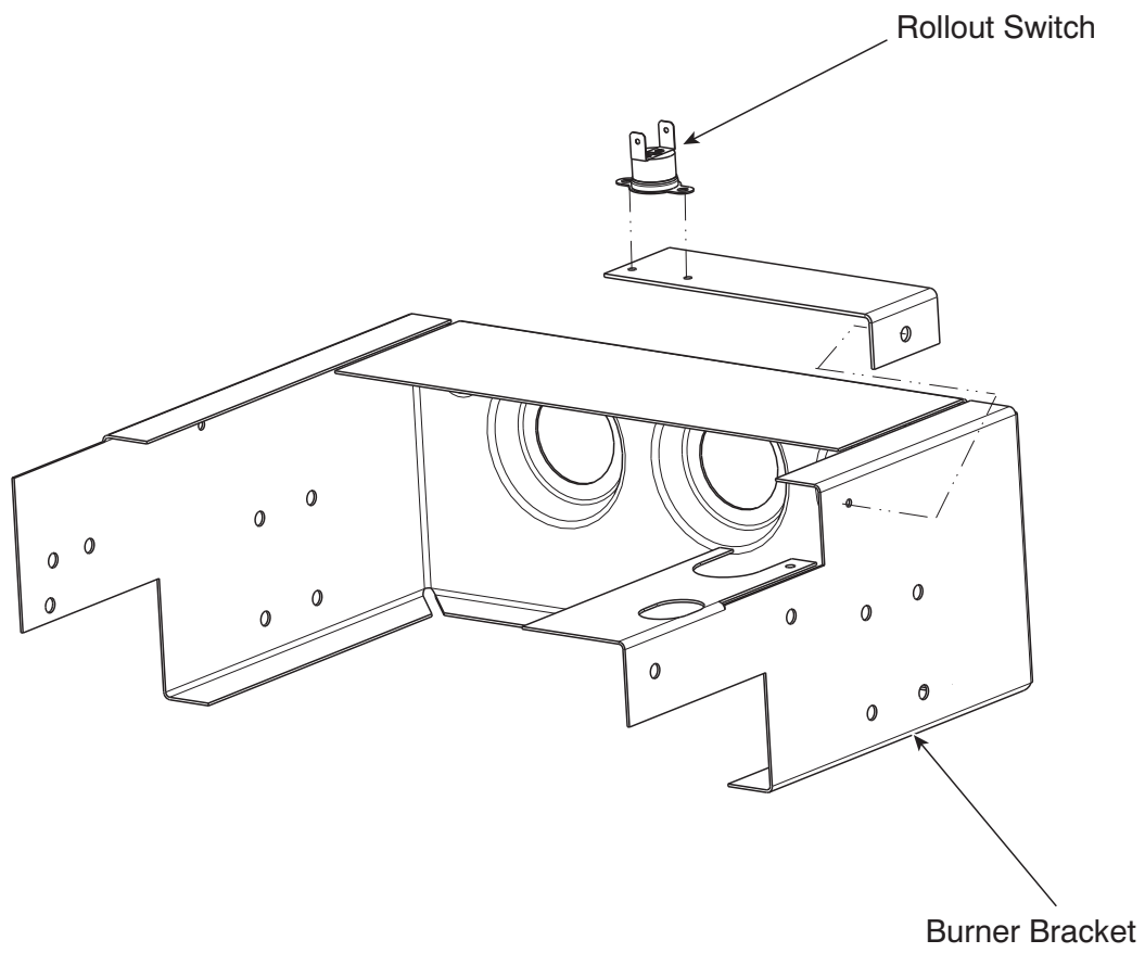
Fig. 17 - Single-Stage Burner Bracket
