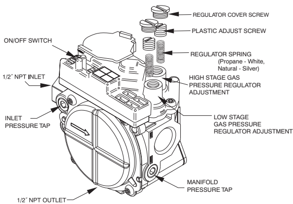
Fig. 3 - Two-Stage Gas Valve
