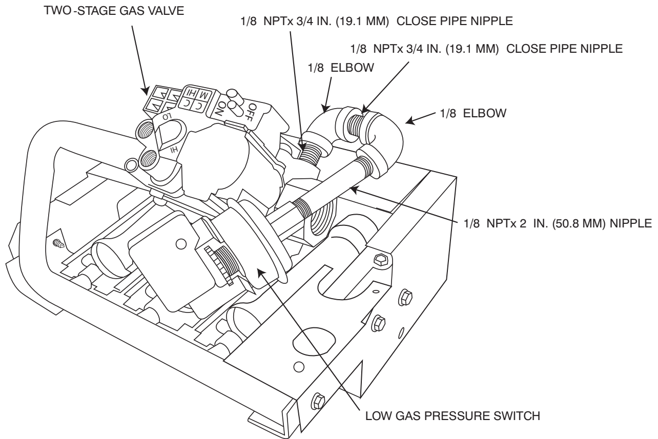
Fig. 10 - Installing Elbows, Nipples, and Pressure Switch on Two-Stage Units
