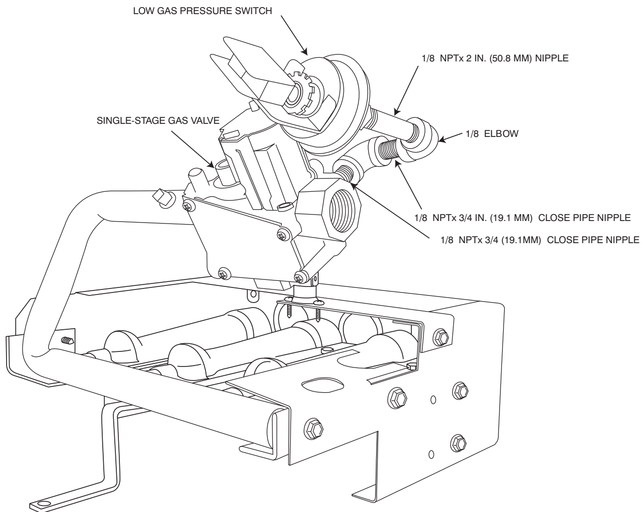
Fig. 18 - Installing Elbows, Nipples, and Pressure Switch on Single-Stage Units
