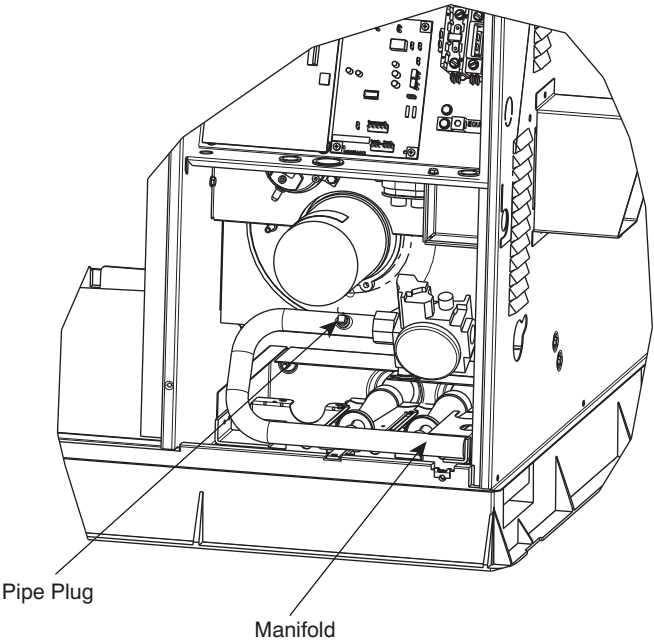
Fig. 14 - Single-Stage Burner Assembly
