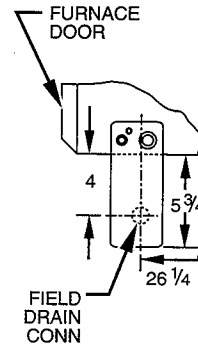
END VIEW
