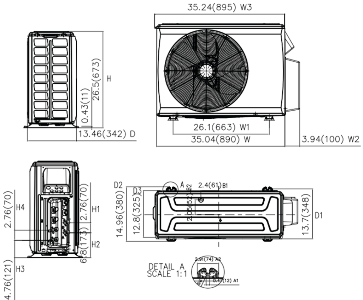
Fig. 4 — Outdoor Dimensions Size 18R (Standard)
