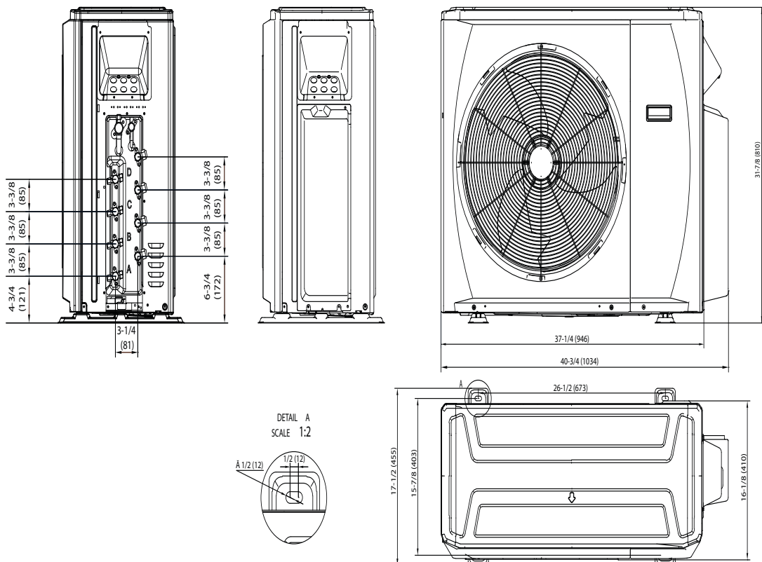
Fig. 6 — Outdoor Dimensions Sizes 30HH (High Heat) and 36R (Standard)
