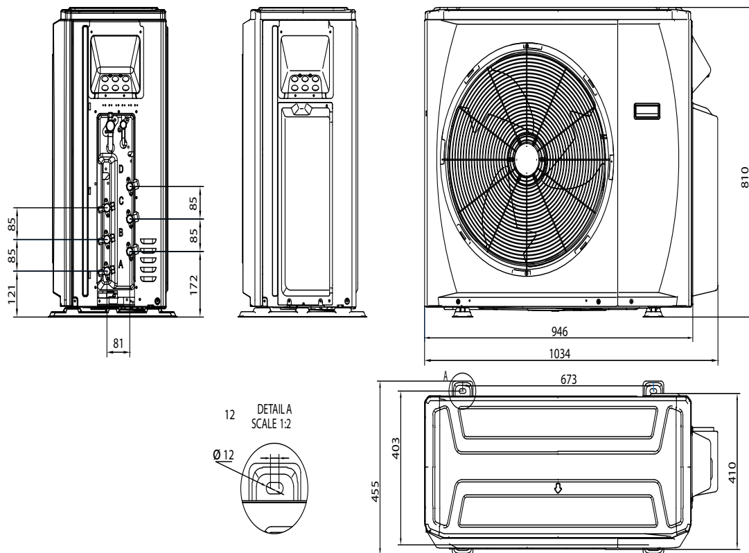
Fig. 5 —Outdoor Dimensions Size 24HH (High Heat)
