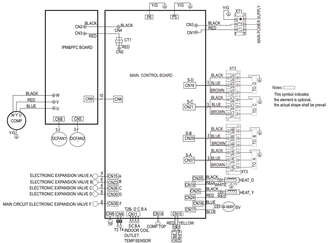
Fig. 5 — Wiring Diagram 36HH (High Heat) - 4 Zone Max
