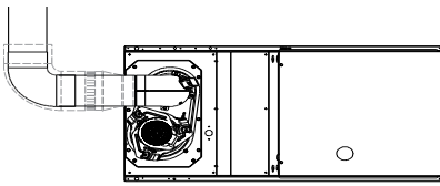
Downflow Application-Vent Elbow Left then Up
