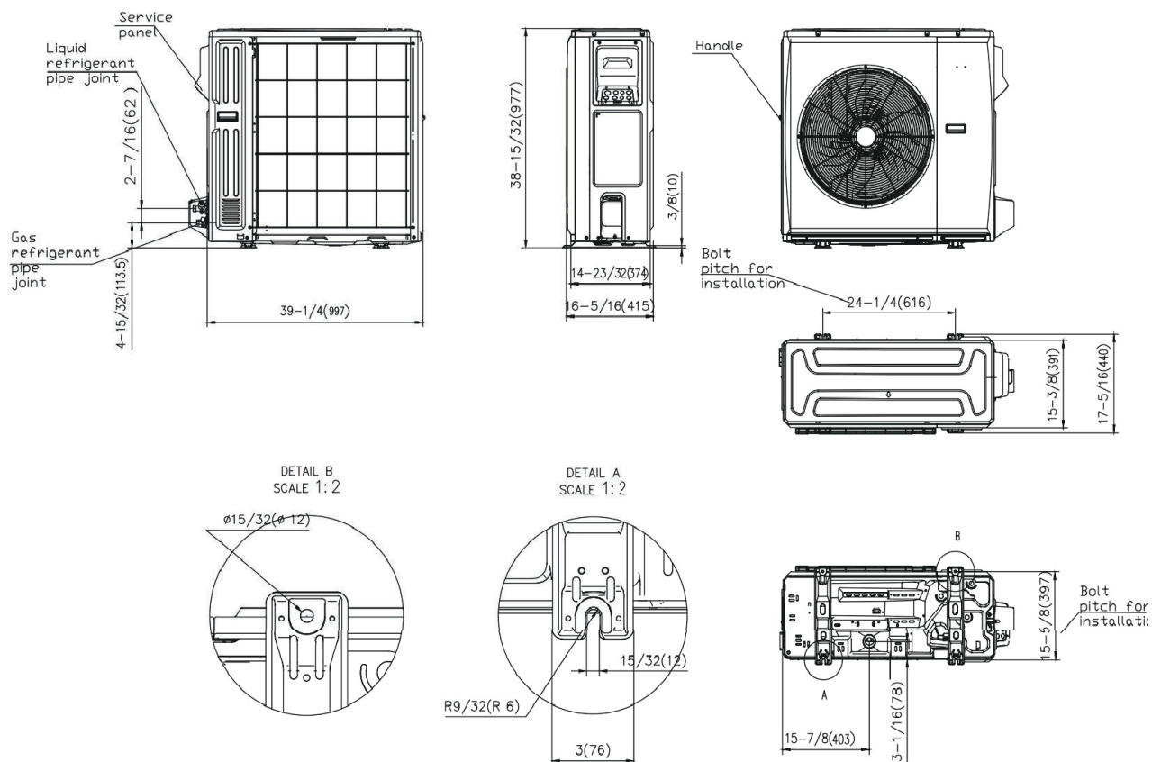
Fig. 3 – Outdoor Dimensions Size 36K
