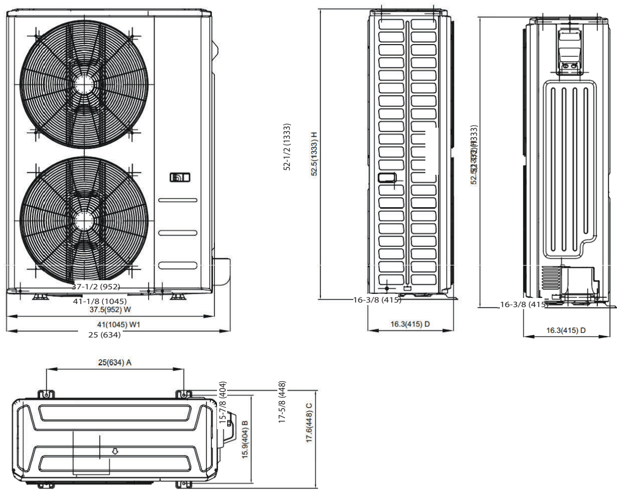
Fig. 4 – Outdoor Dimensions Size 48K and 58K
