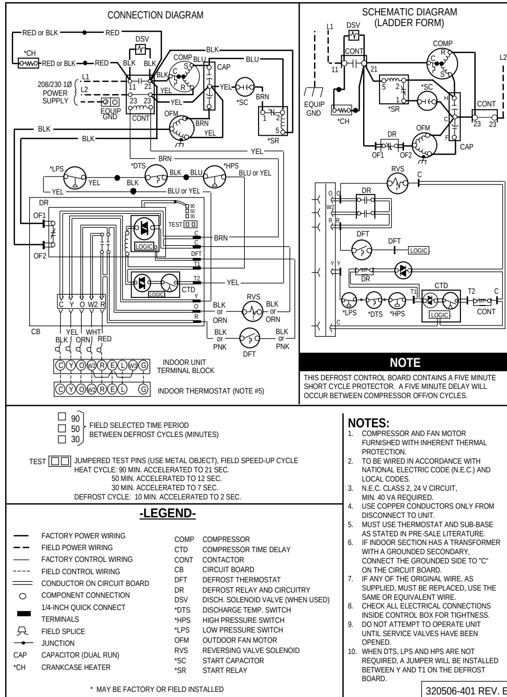
Fig. 1—38YRA018-042 (A,B); 048 (A) 208/230v, 1 Phase, 60 Hertz
