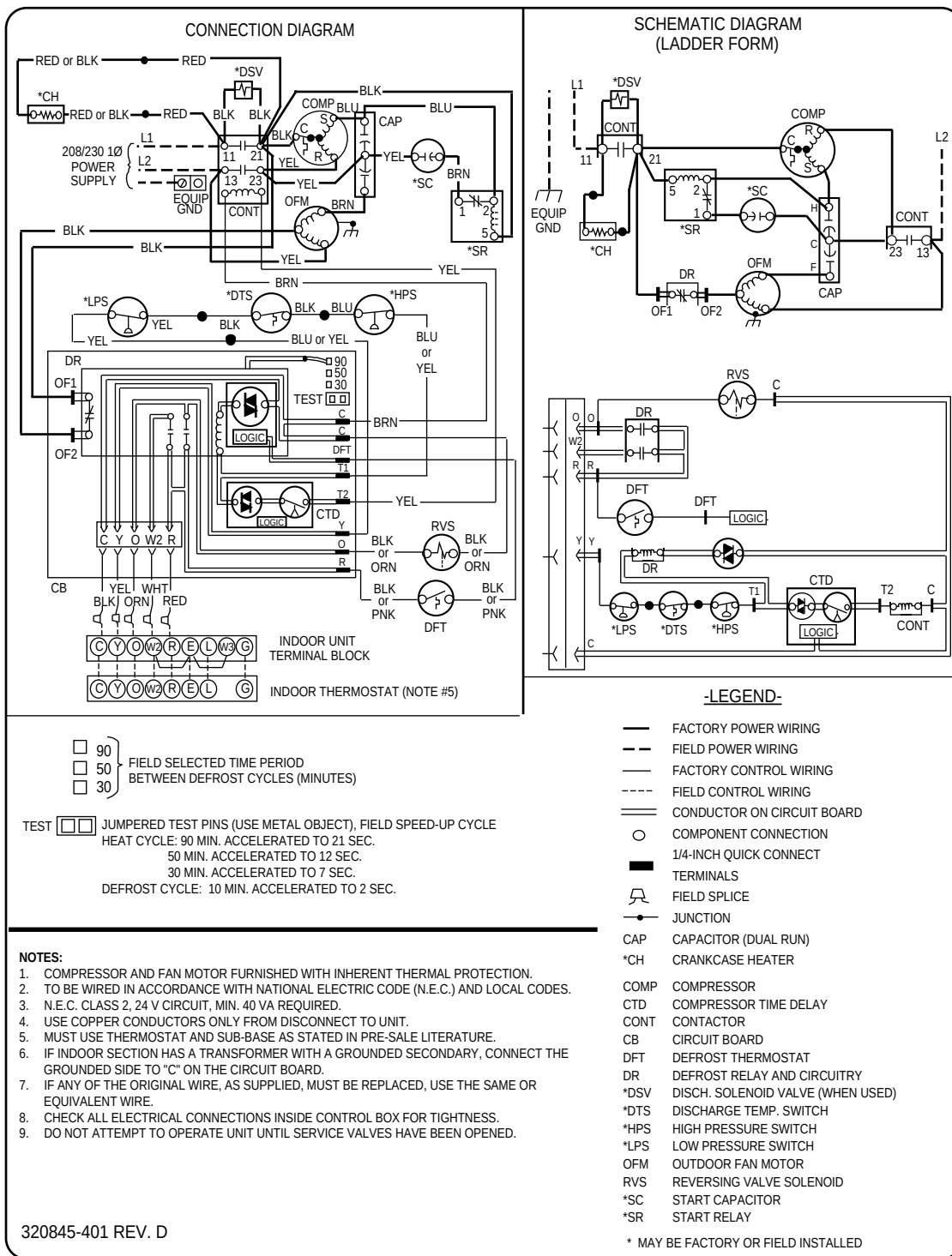
Fig. 2—38YRA060 (A) 208/230v, 1 Phase, 60 Hertz
