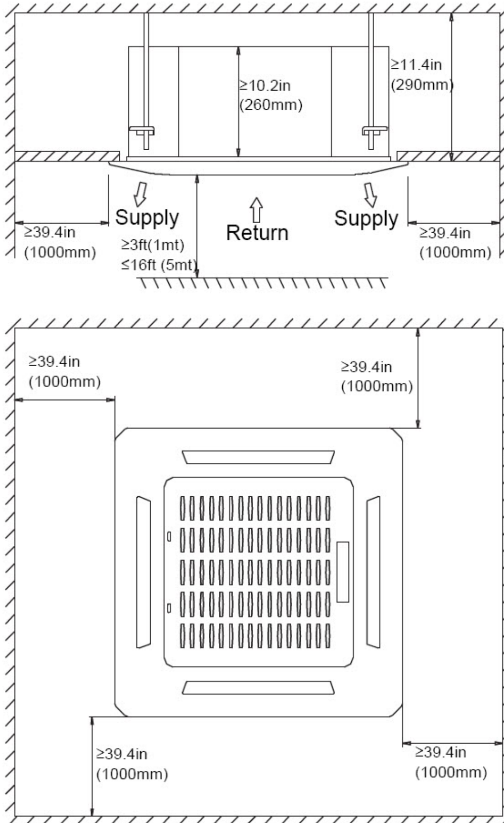
Fig. 6 — Clearances
