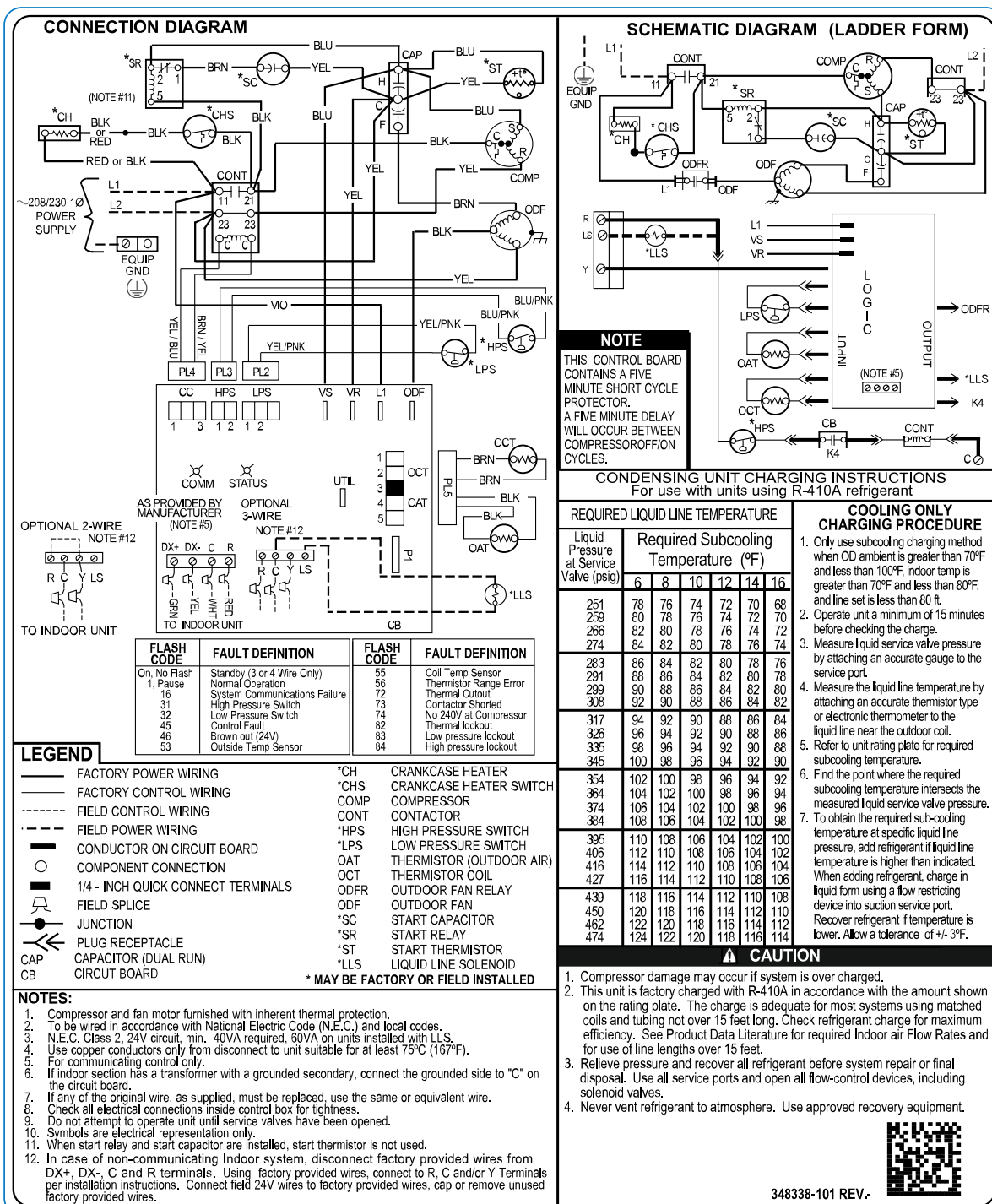
Fig. 1 – 18-60 Wiring Diagram
