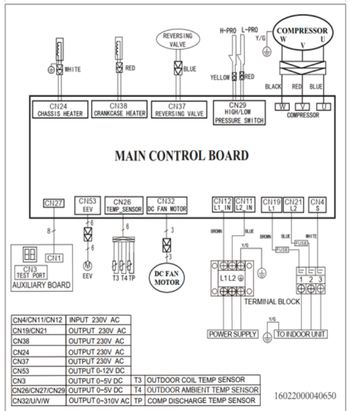
Fig. 11 – 36K – 208/230V Wiring Diagram
