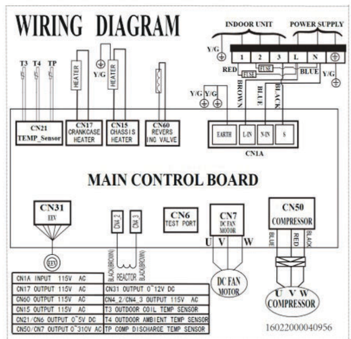
Fig. 7 – 12K – 115V Wiring Diagram
