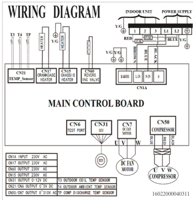
Fig. 8 – 9K/12K – 208/230V Wiring Diagram
