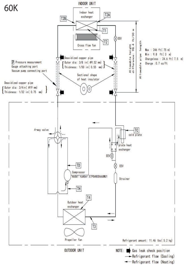
Fig. 28 — Refrigerant Cycle 48K. 60K
