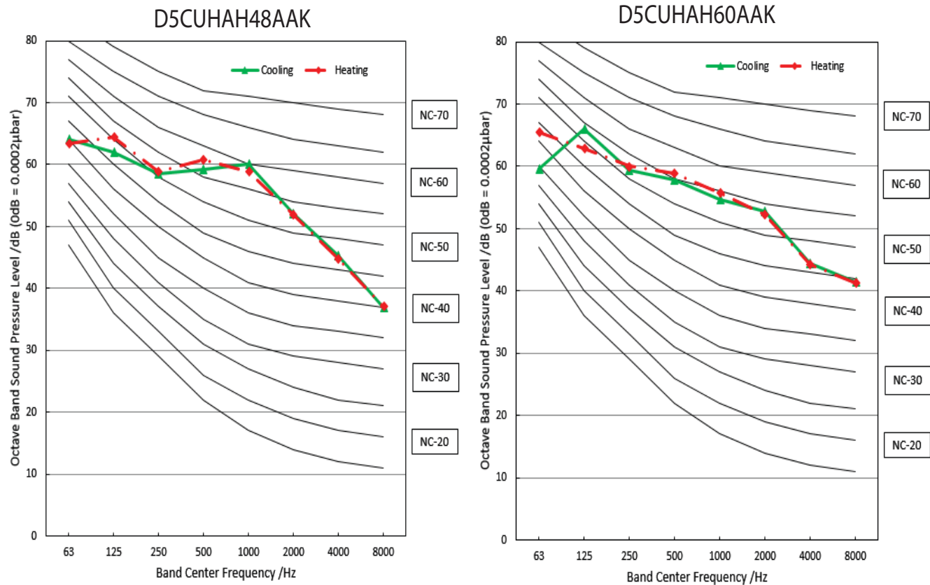
Fig. 19 —Sound Octave Bands
