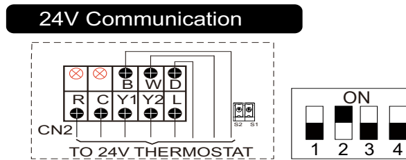
Fig. 15 —Scenario 3 - Wiring to the Outdoor Unit
