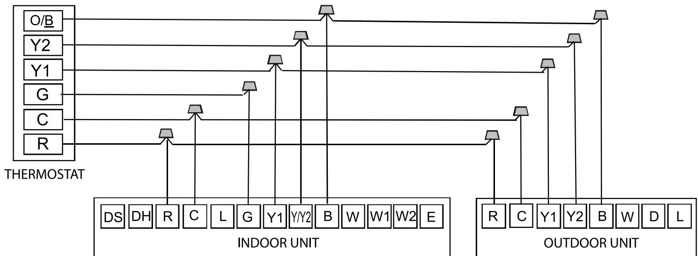
Fig. 32 —Wiring for 2H and 2C thermostat
