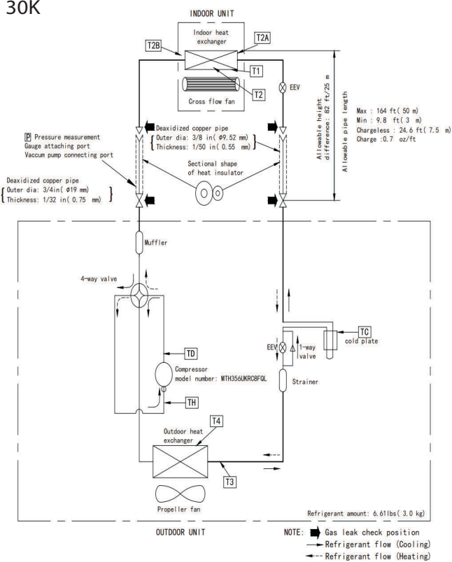
Fig. 27 —Refrigerant Cycle 30K, 36K
