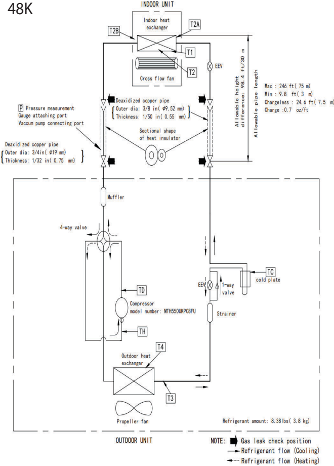
Fig. 28 — Refrigerant Cycle 48K. 60K
