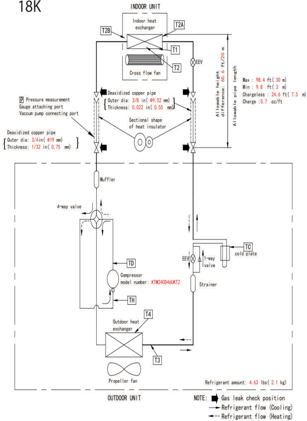
Fig. 26 —Refrigerant Cycle 18K, 24K
