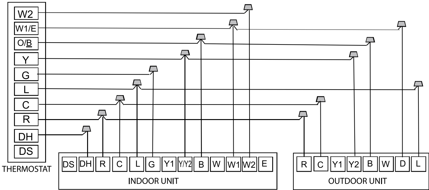
Fig. 29 —Wiring for 4H and 2C thermostat
