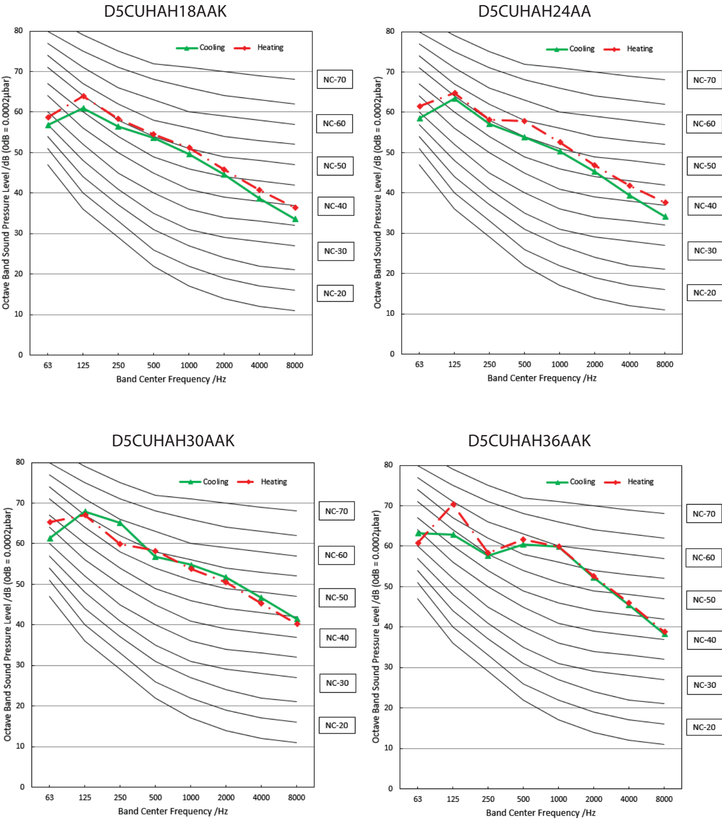
Fig. 18 — Sound Octave Bands
