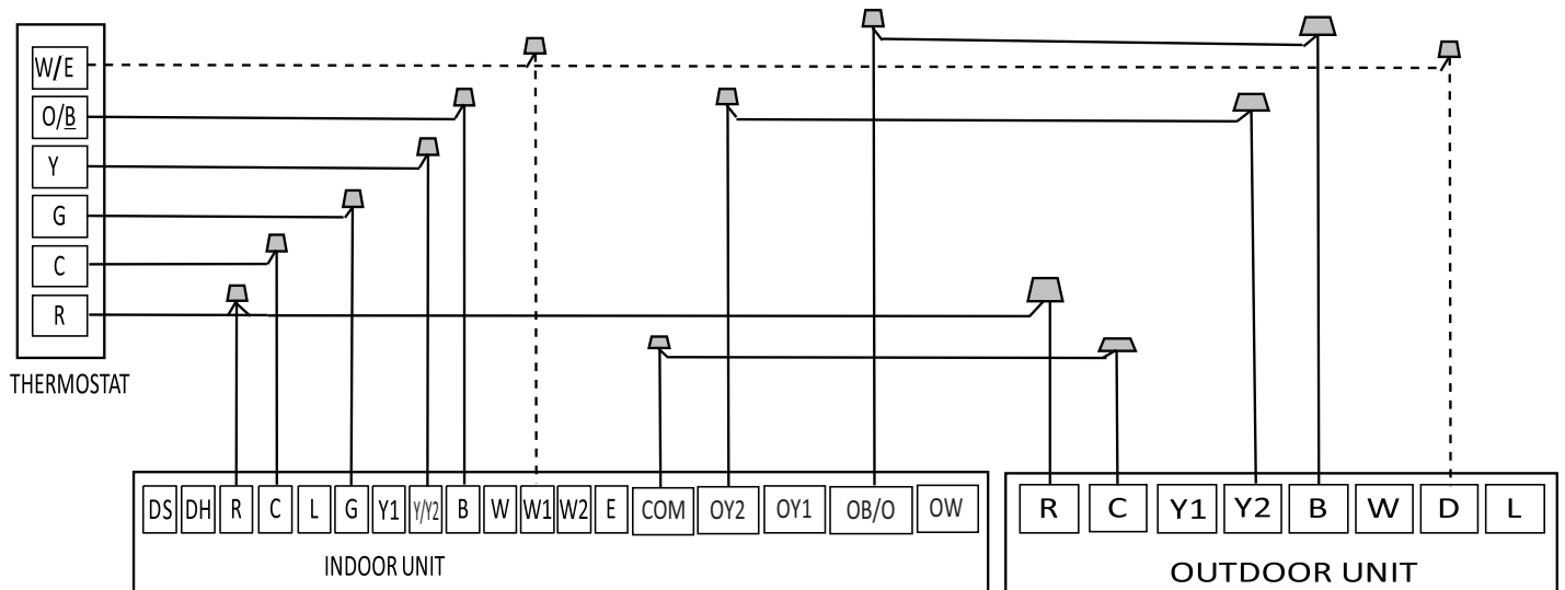
Fig. 33 —Wiring for 3H and 2C thermostat
