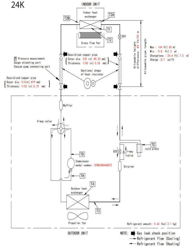
Fig. 26 —Refrigerant Cycle 18K, 24K
