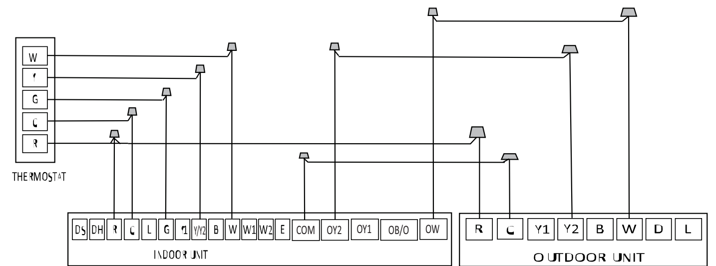
Fig. 36 —Wiring for 1H and 1C thermostat
