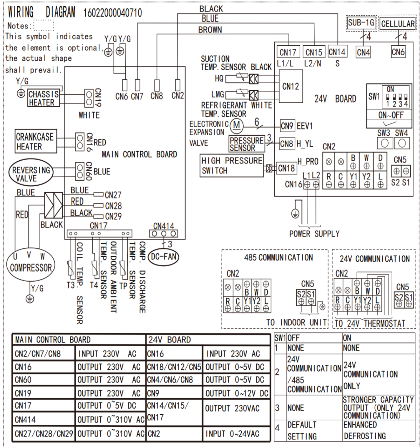
Fig. 37 — Wiring Diagram Sizes 18K and 24K
