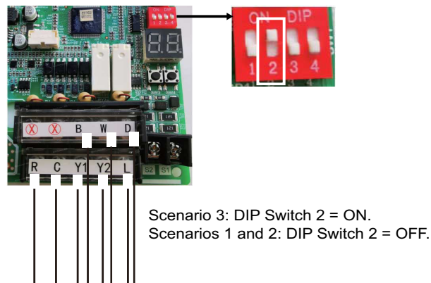
Fig. 16 —24V Connection Dip Switch Setting (as shown in Fig 15)
