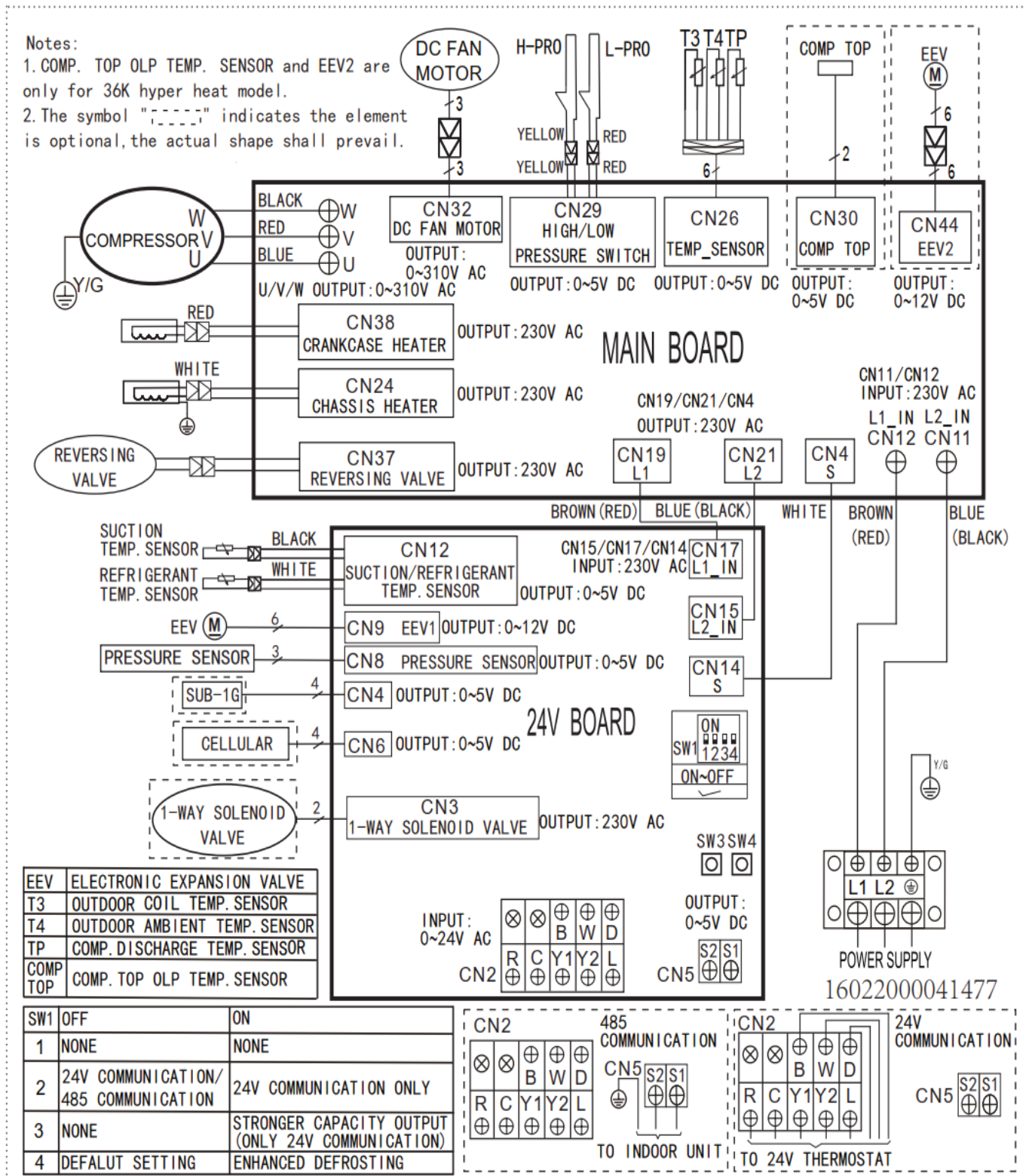
Fig. 39 — Wiring Diagram Sizes 36K - 48K
