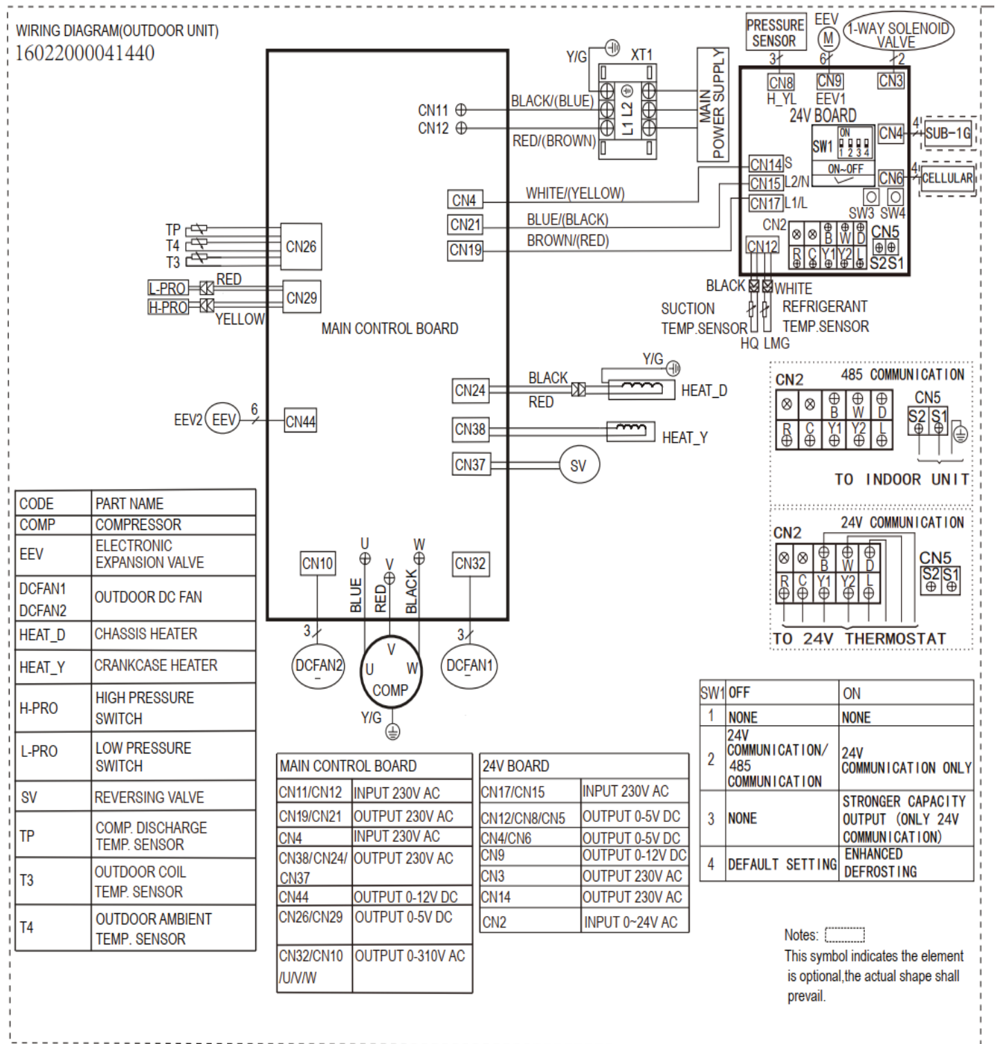
Fig. 40 — Wiring Diagram Size - 60K
