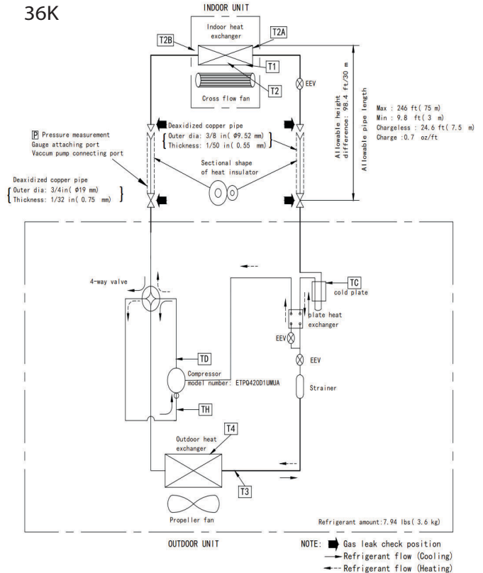
Fig. 27 —Refrigerant Cycle 30K, 36K
