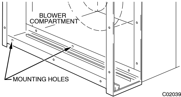
Fig. 7 – Mounting Holes
