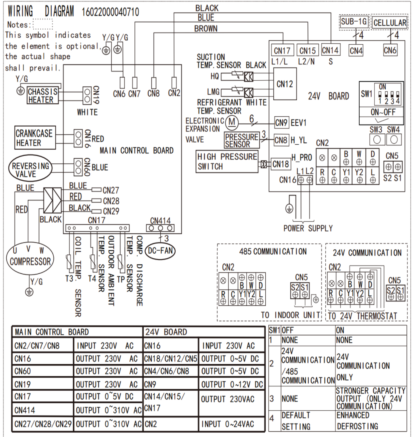
Fig. 37 — Wiring Diagram Sizes 18K and 24K
