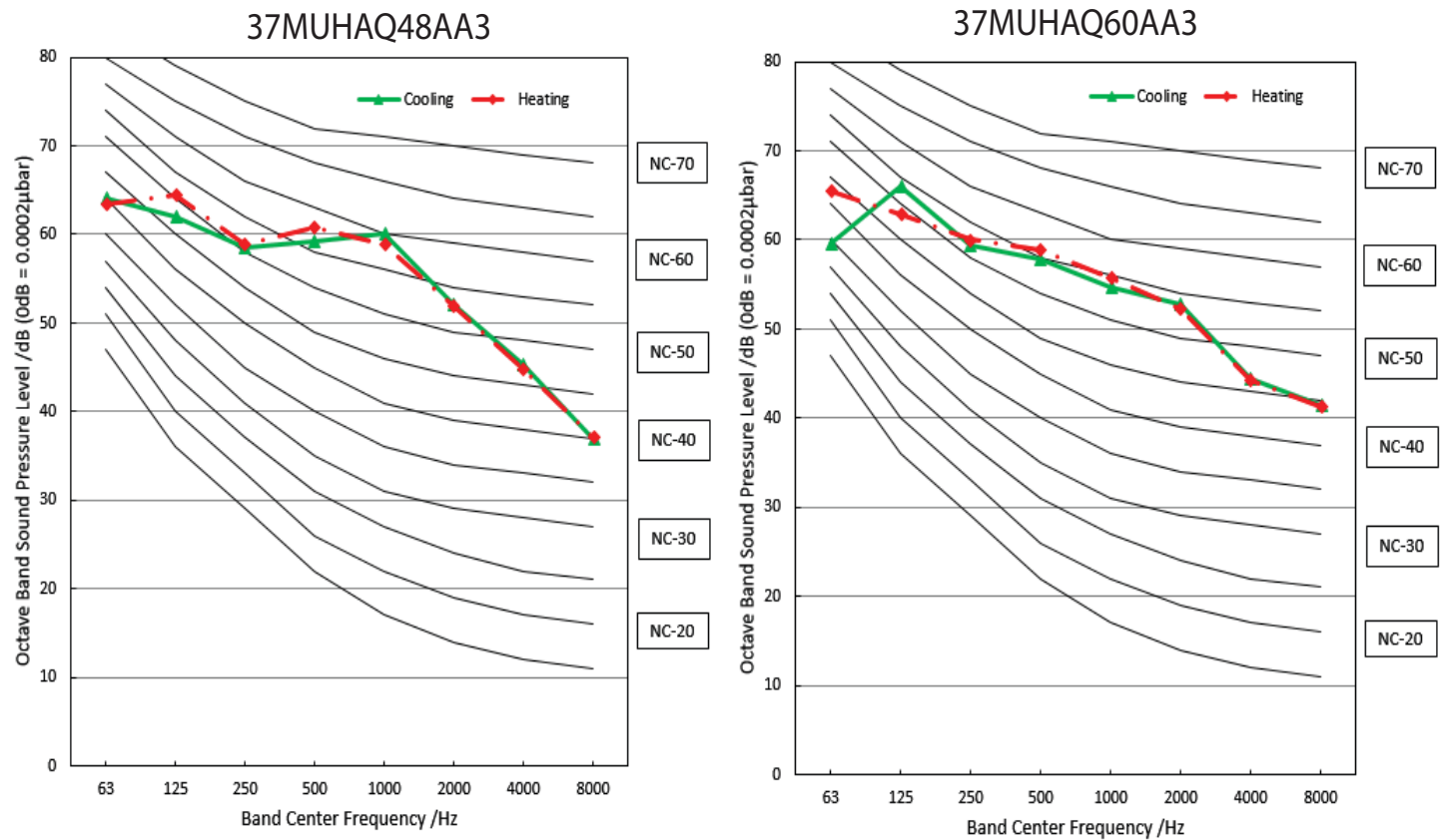
Fig. 19 —Sound Octave Bands
