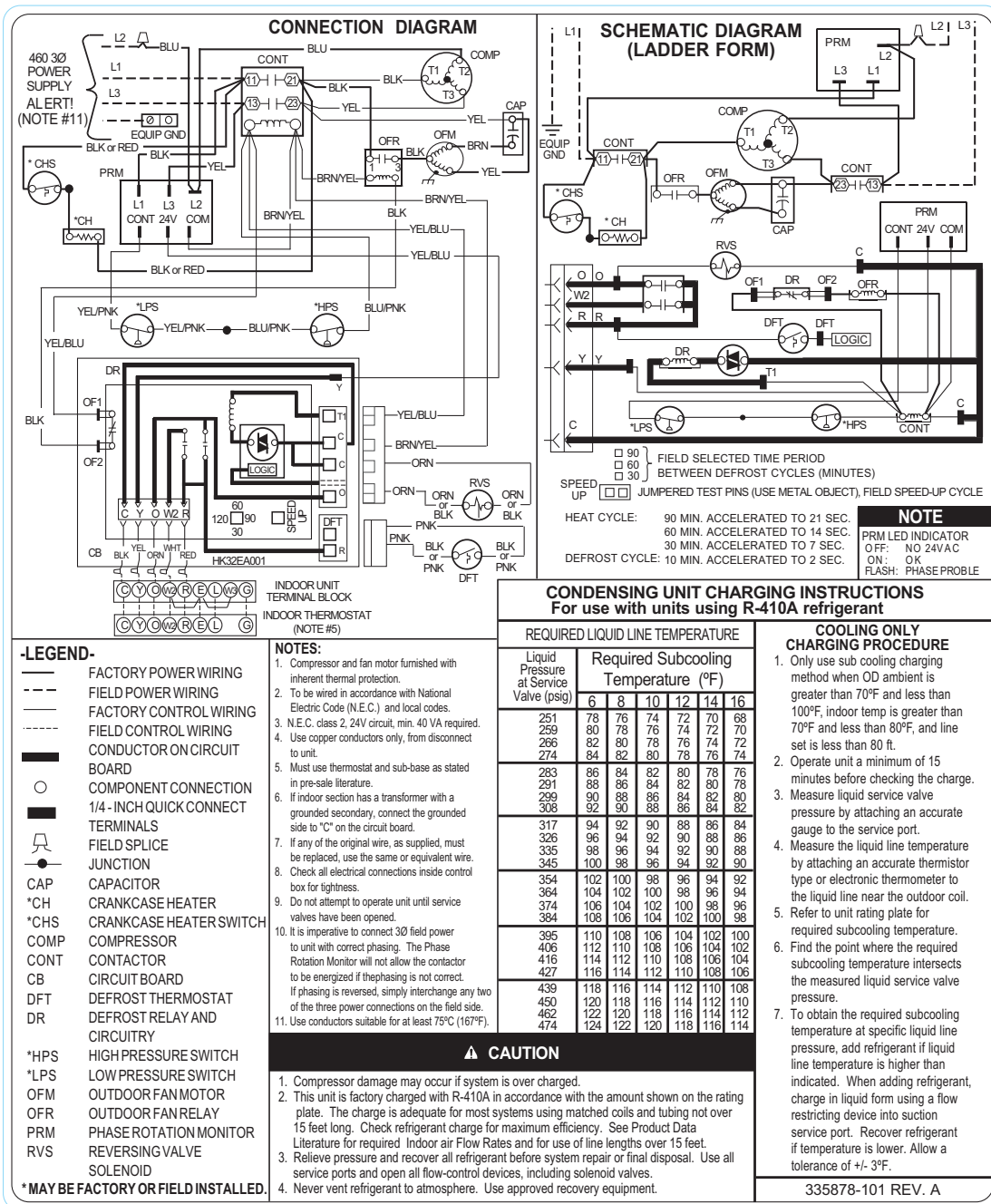
Fig. 3 – Wiring Diagram — Model size 3 - 5 tons, 460/3
