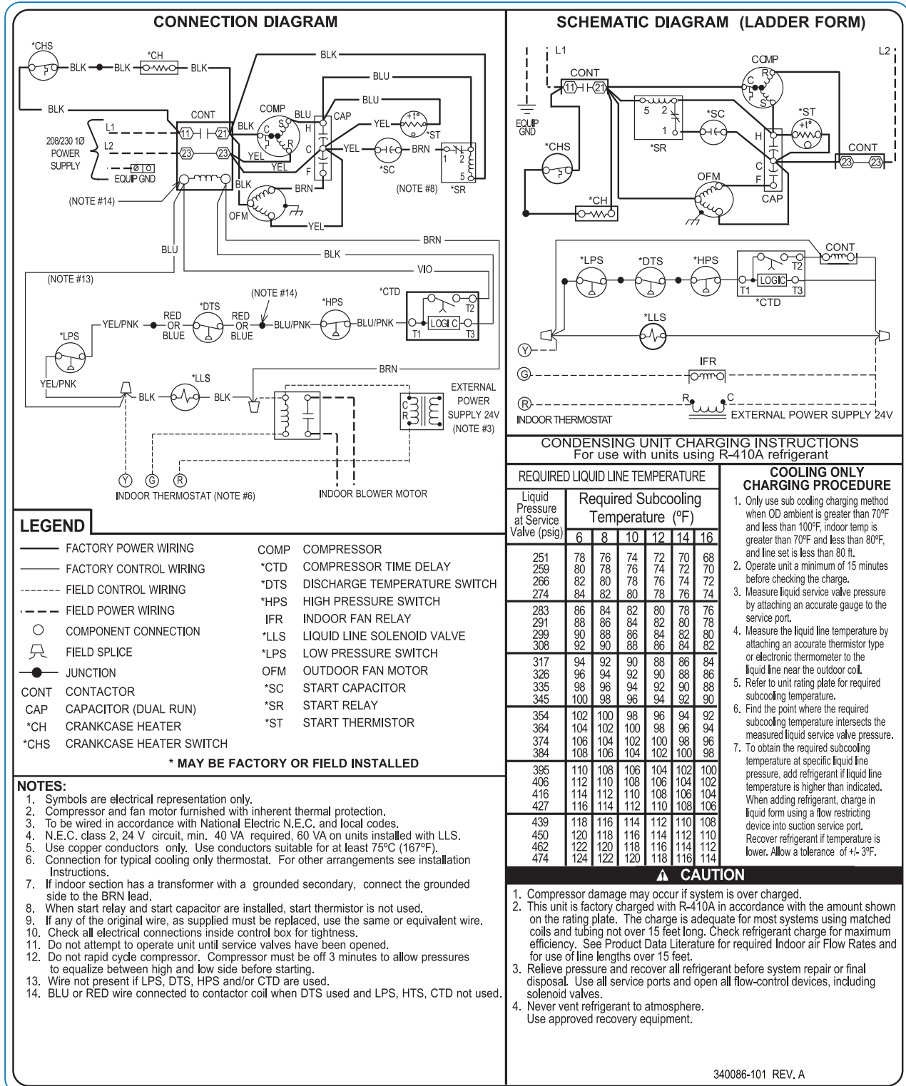
Fig. 1 – Wiring Diagram — Model sizes 1-1/2 - 5 Tons, 208/230-1
