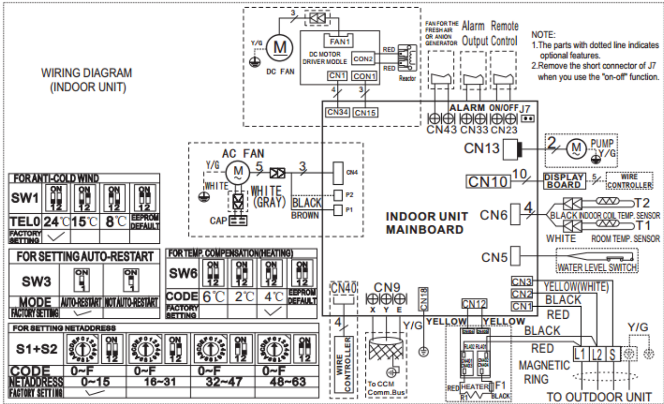
Fig. 20 — Wiring Diagram Sizes 9K - 24K
