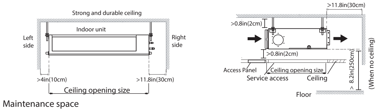
Fig. 5 — Installation Clearances
