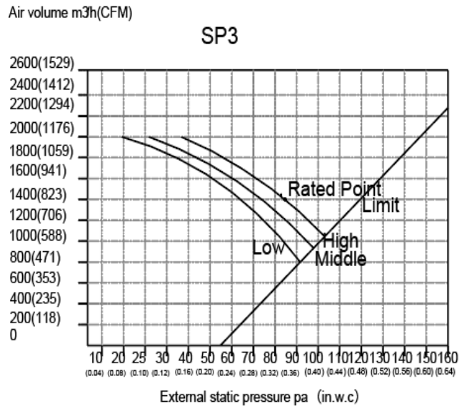
Fig. 18 — Fan Performance - DLFLDAH48XAK
