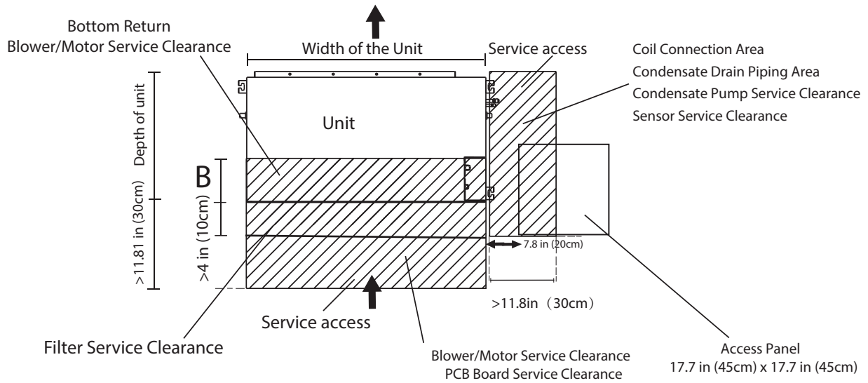
Fig. 6 — Maintenance Clearances
