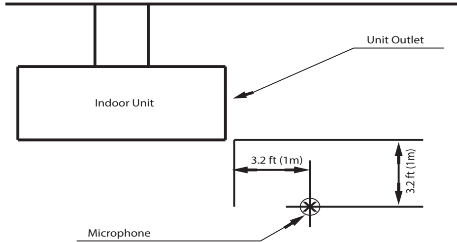
Fig. 10 — Sound Pressure Testing Method
