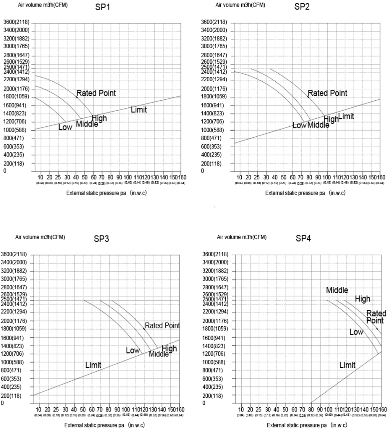
Fig. 17 — Fan Performance - DLFLDAH36XAK
