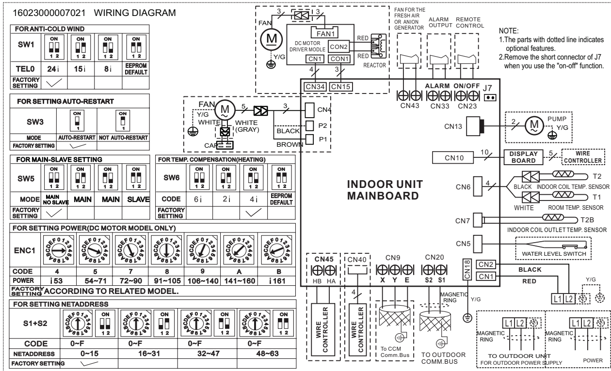
Fig. 22 — Wiring Diagram Size 58K
