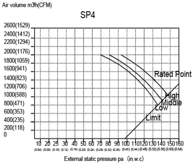
Fig. 18 — Fan Performance - DLFLDAH48XAK
