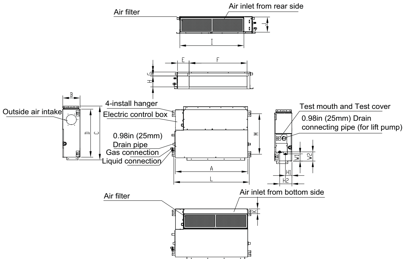
Fig. 3 — Indoor Unit Sizes 9K - 48K
