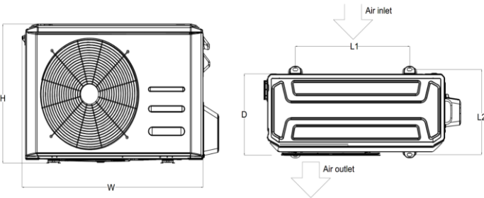
OUTDOOR UNIT DIMENSIONS
