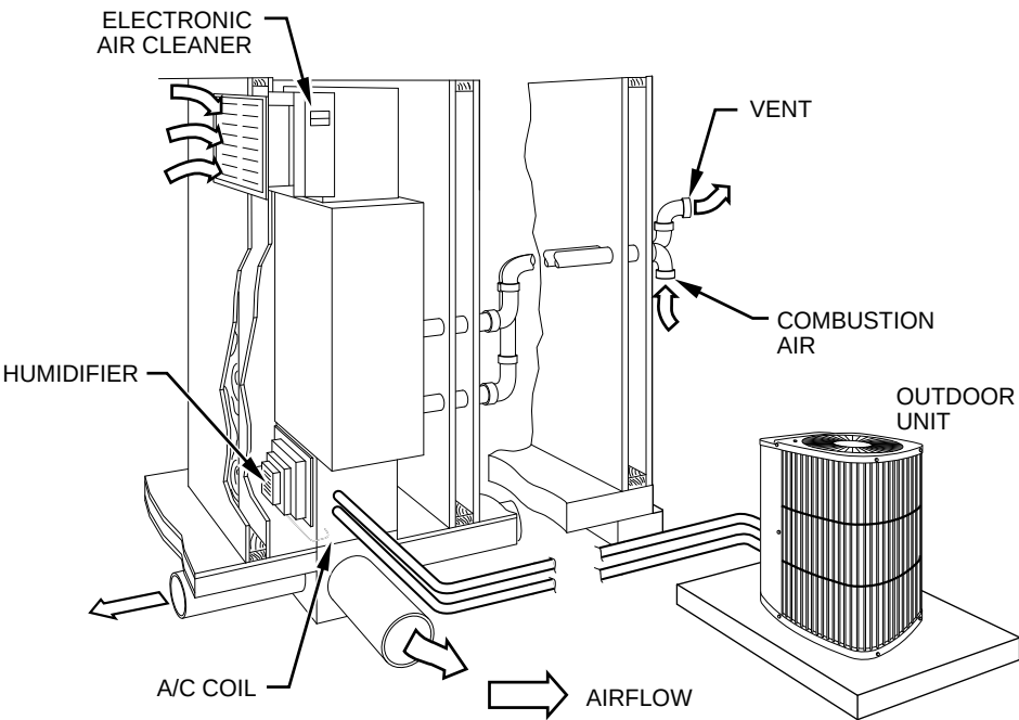
Closet — Downflow Application
