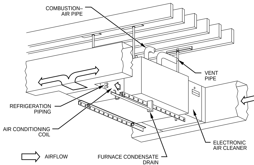
Crawlspace — Horizontal Application
