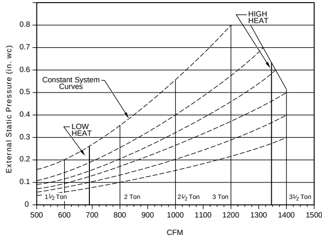
AIR DELIVERY CURVE — 080-14
