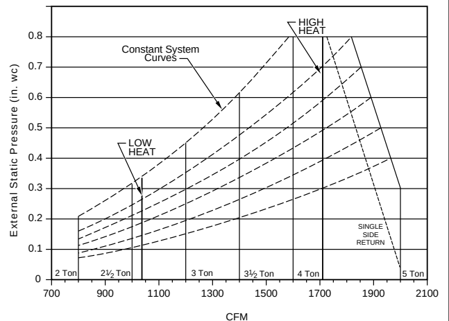
AIR DELIVERY CURVE — 120-20
