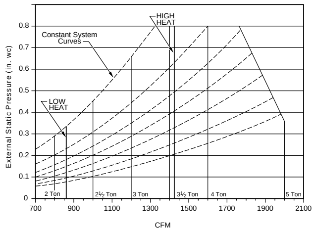
AIR DELIVERY CURVE — 100-20
