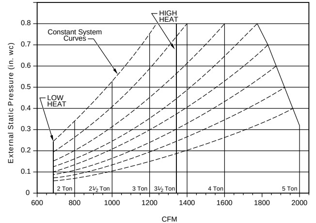
AIR DELIVERY CURVE — 080-20
