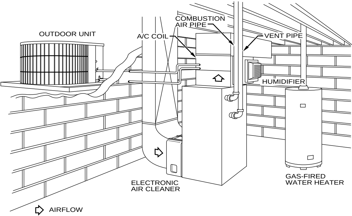
Basement — Upflow Application
