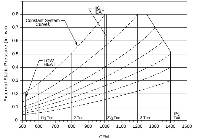
AIR DELIVERY CURVE — 060-14
