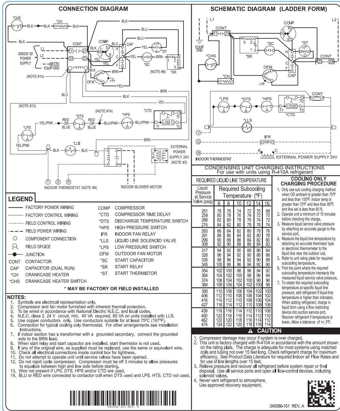
Fig. 1 – Wiring Diagram — Models CA13NA, CA14NA, CA15NA, CA16NA Sizes 024-060, CA16NW Sizes 018-060, 208/230-1
