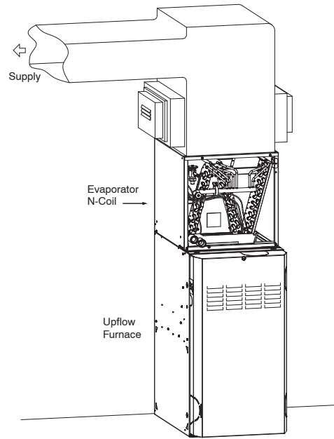
Fig. 7 - Installation of Humidifier in System with N-Coil
