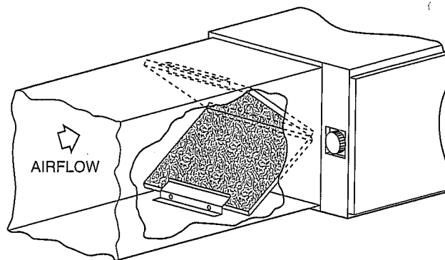
Filter Retainers (Field Supplied)
