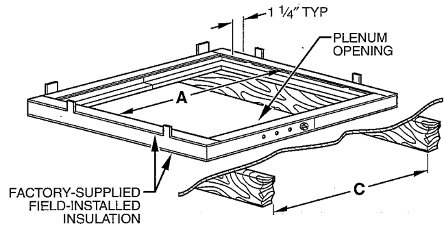
Assembled
