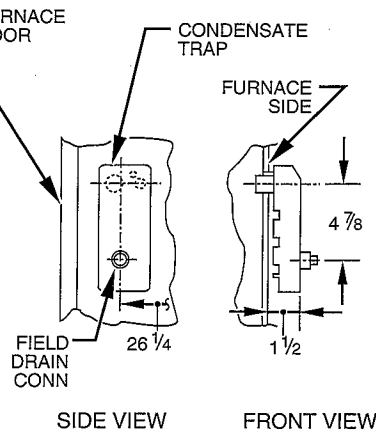
SIDE VIEW FRONT VIEW DOWNFLOW AND ALTERNATE EXTERNAL UPFLOW APPLICATIONS
