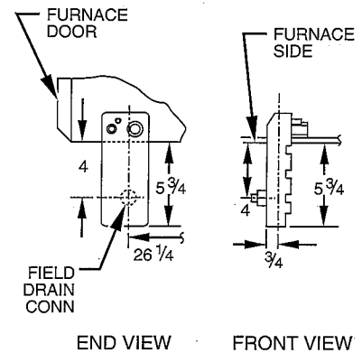
END VIEW FRONT VIEW HORIZONTAL APPLICATIONS
