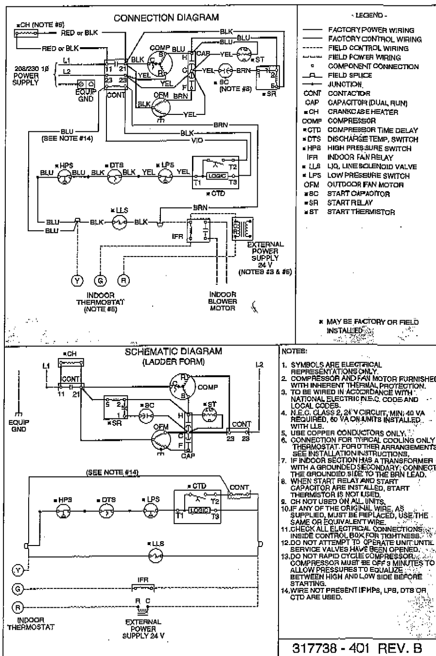
Fig. 1—PA12NA024-048 208-230v, 1 Phase, 60 Hertz
