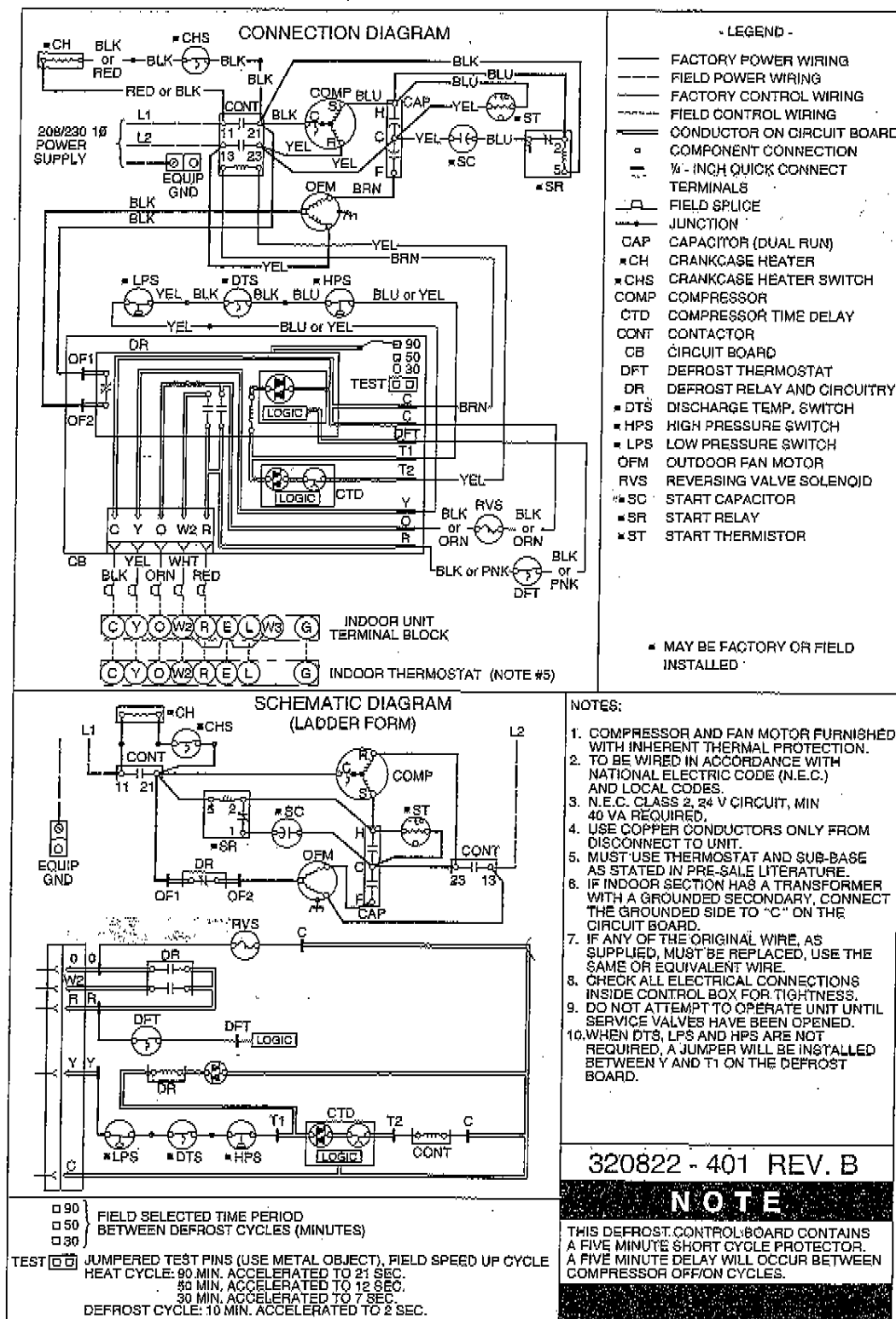
Fig. 2—PH12NA 060-A 208/230v, 1 Phase, 60 Hertz
