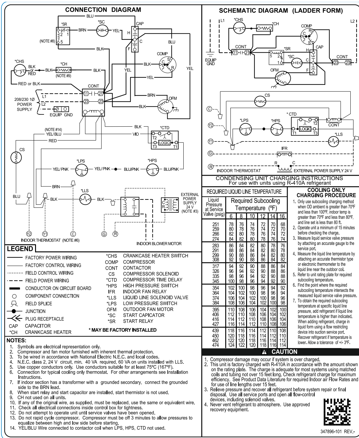
Fig. 1 – 208/230-1 - Model Sizes 24 - 60
