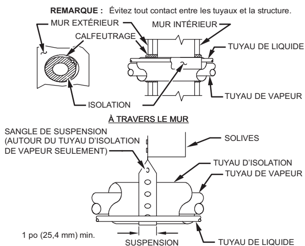
Figure 1 – Installation de la tuyauterie
