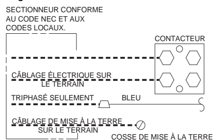
Figure 5 – Raccords de conduite
