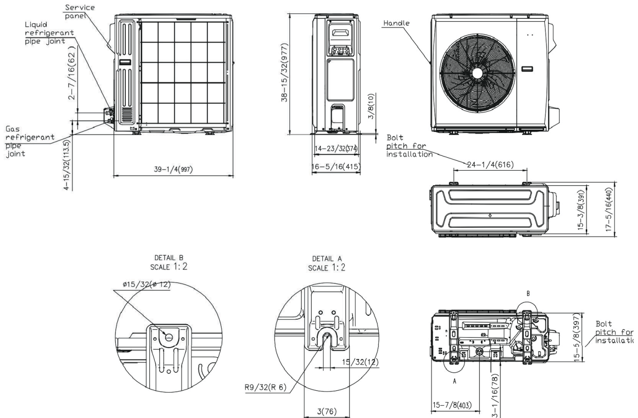
Fig. 3 – Outdoor Dimensions Size 36K
