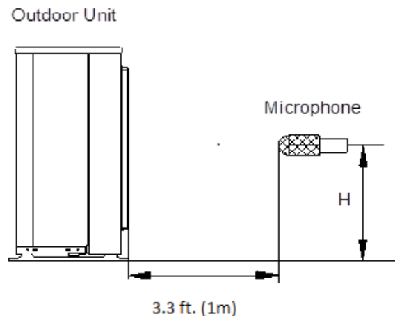
Fig. 7 – Outdoor Unit Sound Pressure Test Conditions
