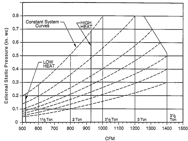
AIR DELIVERY CURVE — 042060
