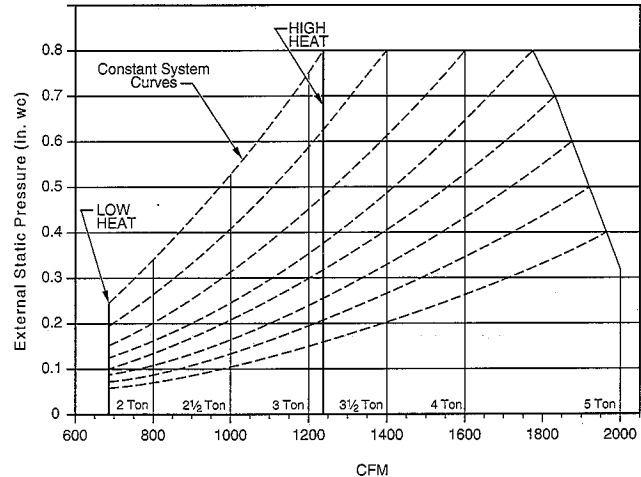
AIR DELIVERY CURVE — 060080
