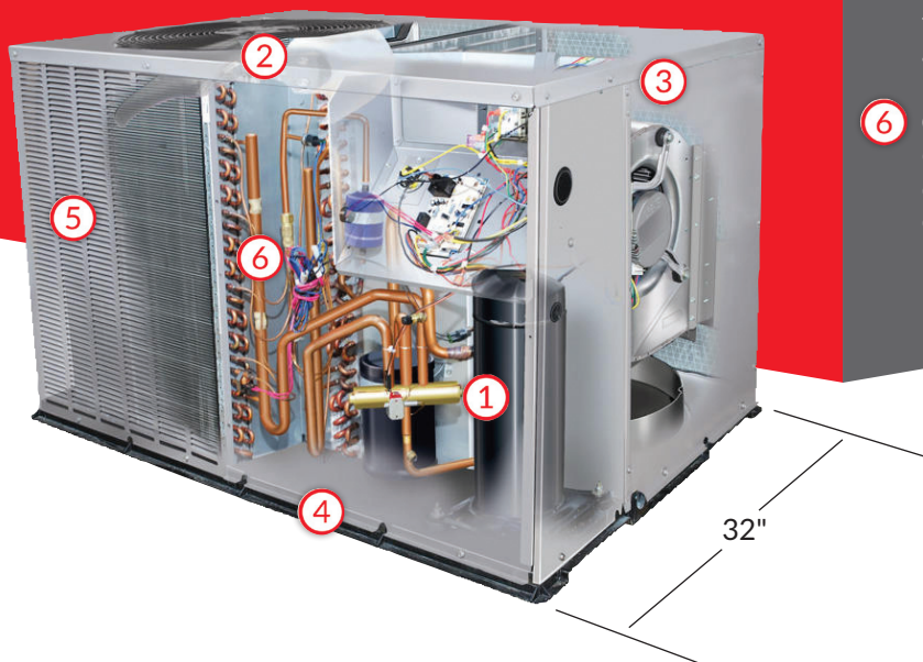
MODEL PH4Z Heat Pump
