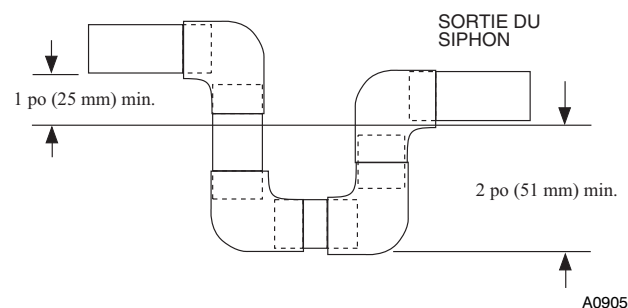
Figure 9 – Siphon de condensat
