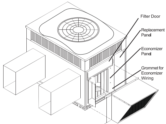
Horizontal Economizer
