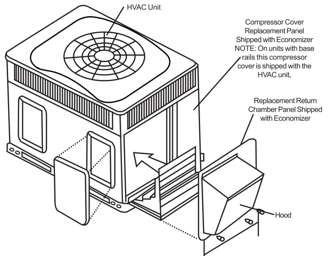
Vertical Economizer
