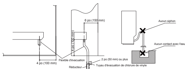
Figure 49 – Siphon
