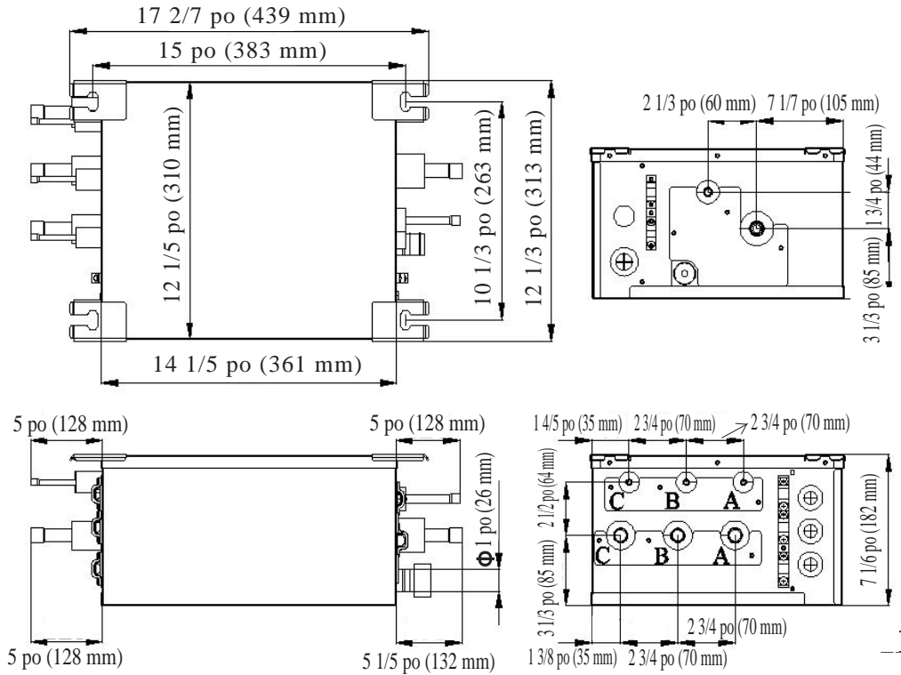
Figure 22 – Dimensions – aperçu
