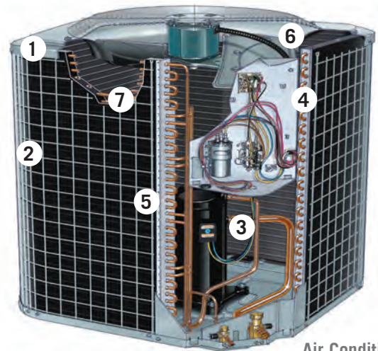
Air Conditioner
