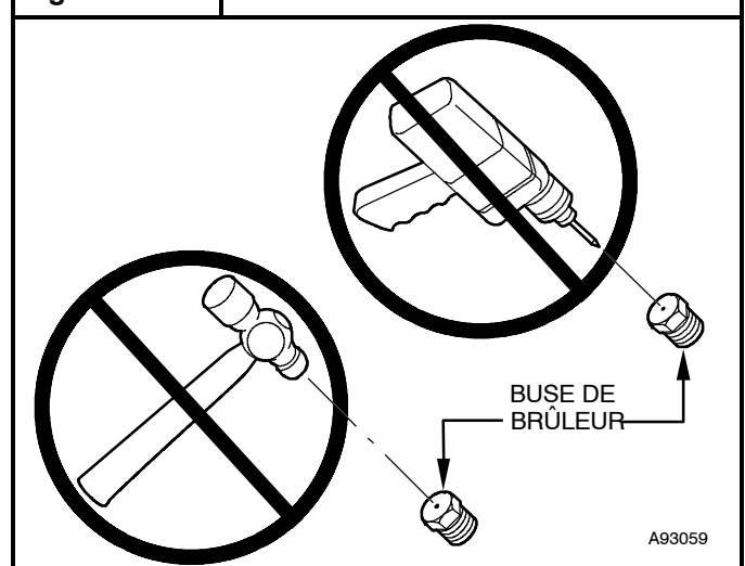
Figure 2 Trou de la buse
