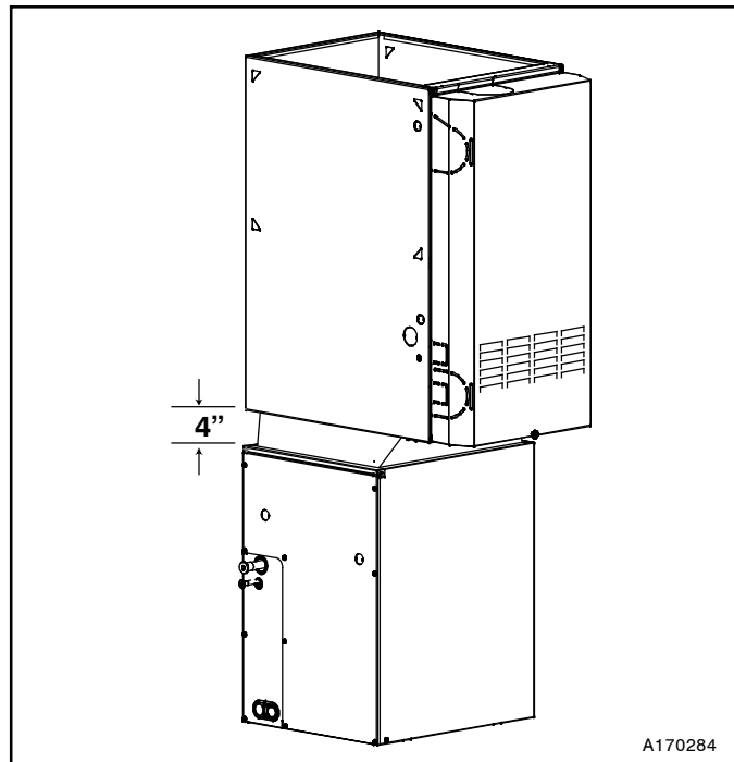
Figure 4 - Downflow Installation with Coil Rotated 90°
