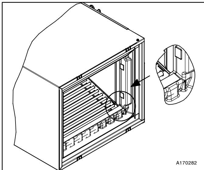
Figure 7 - Condensate Pan Extension Cork Tape Location
