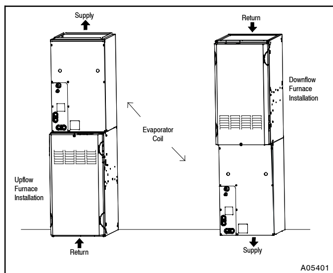
Figure 2 - Typical Coil Installation on Furnace
