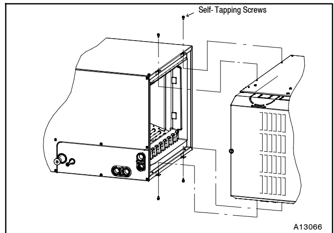
Figure 10 - Horizontal Left Installation
