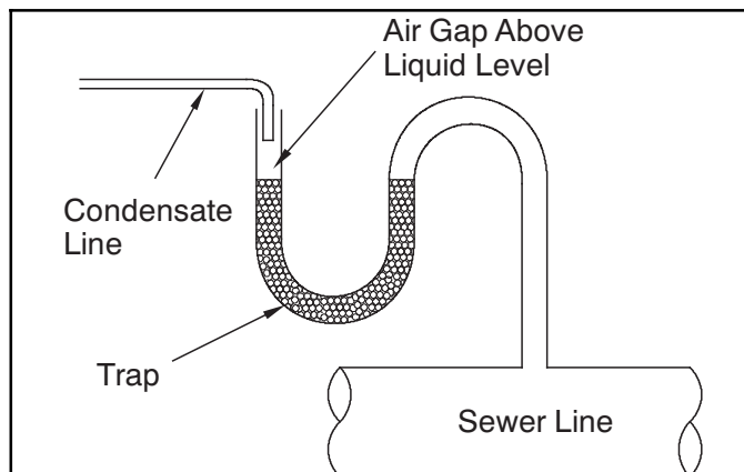
Figure 12 - Condensate Drain to Waste Line
