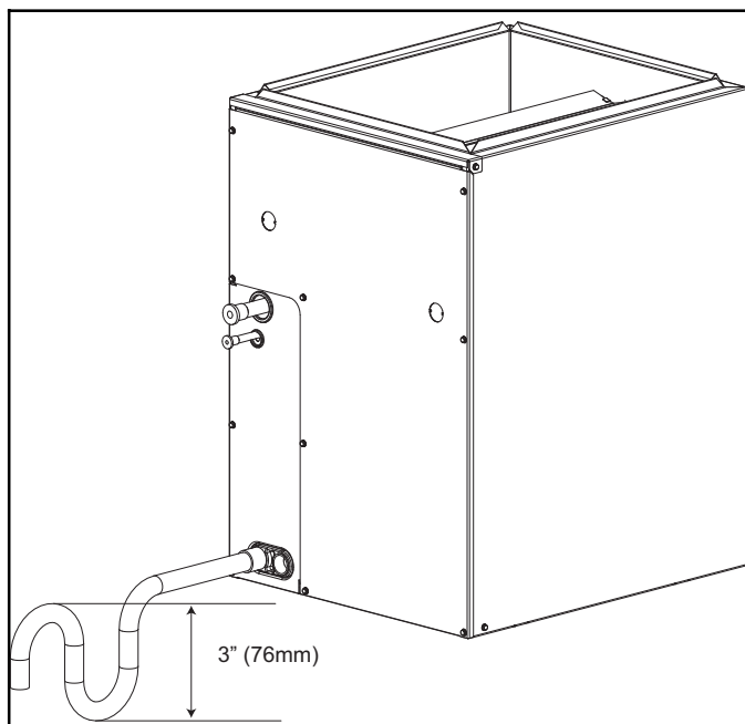
Figure 11 - Condensate Trap
