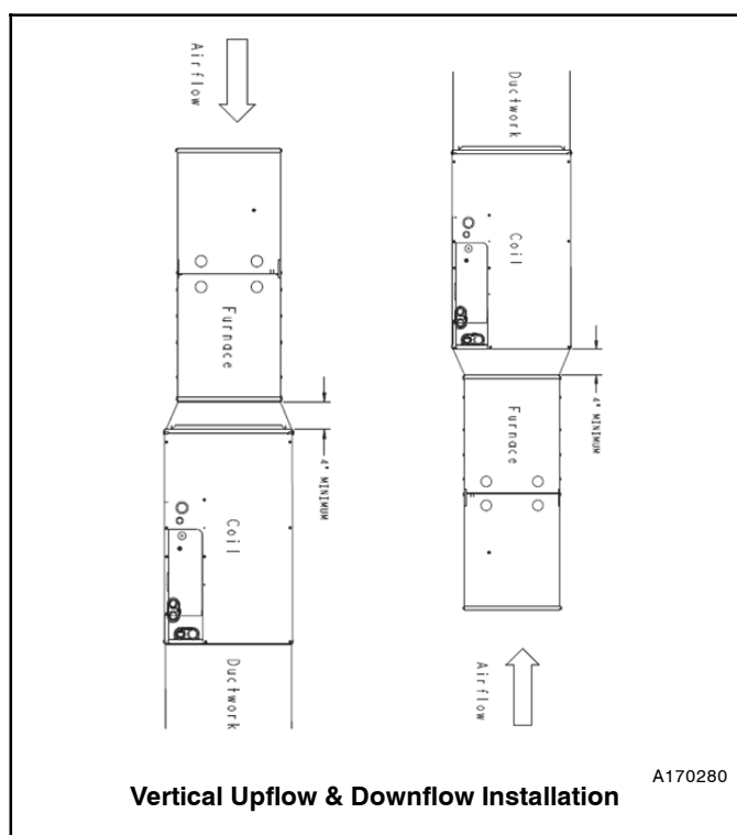
Figure 3 - Adapter(s) Installation When Coil Overhangs Furnace
