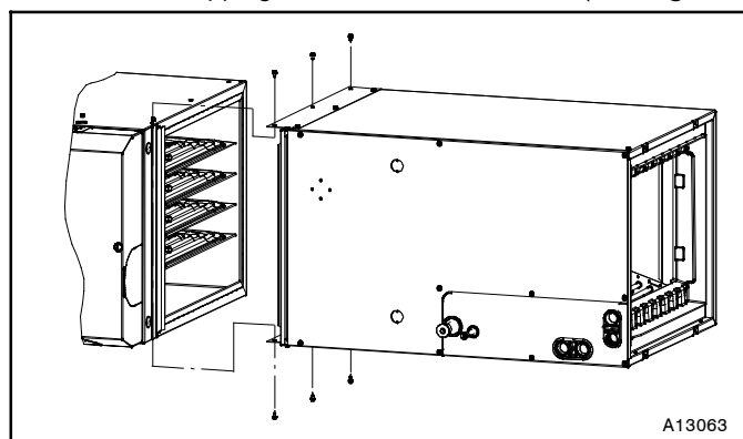
Figure 6 - Horizontal Right Installation
