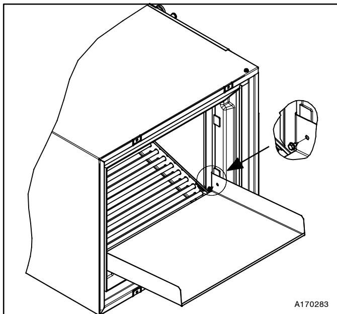
Figure 8 - Condensate Pan Extension Mounting Screws
