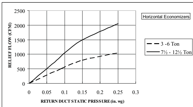
FIGURE 1 – Barometric Relief Flow Capacity C08070
