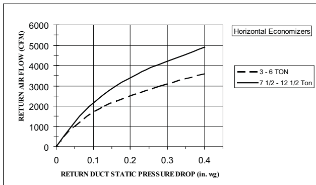
FIGURE 3 – Return Air Pressure Drop C08072
