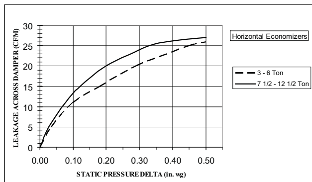
FIGURE 2 – Outdoor Air Damper Leakage C08071
