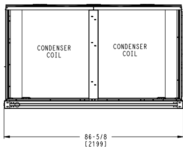
(HORIZONTAL DISCHARGE W/ ECON) (WHEN ORDERED)
