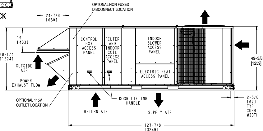
Optional Economizer Hood
