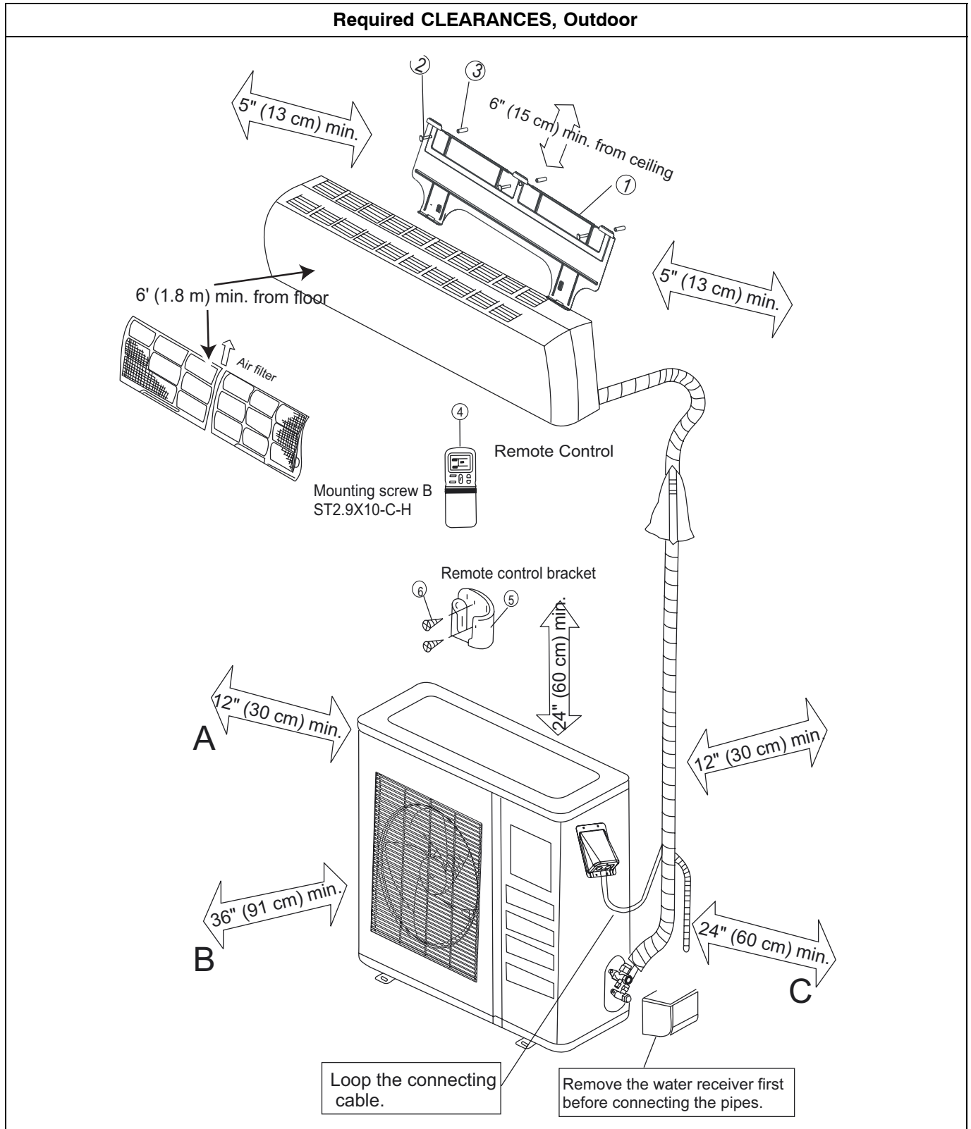
Fig. 2 – DFF4(A/H)H/DFC4(A/H)3 18–24 Parts List and Clearances
