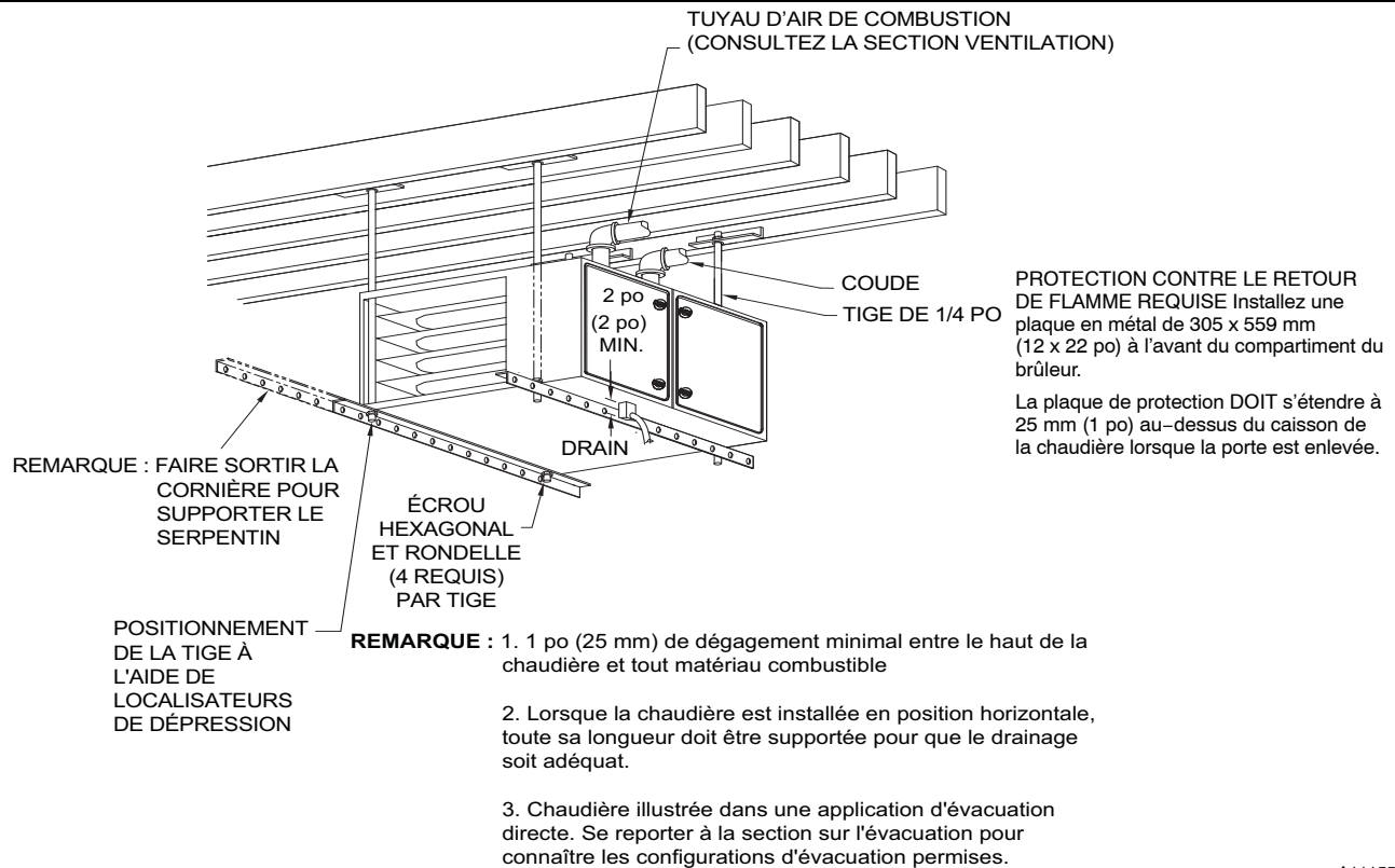
Figure 26 Installation de chaudière suspendue
