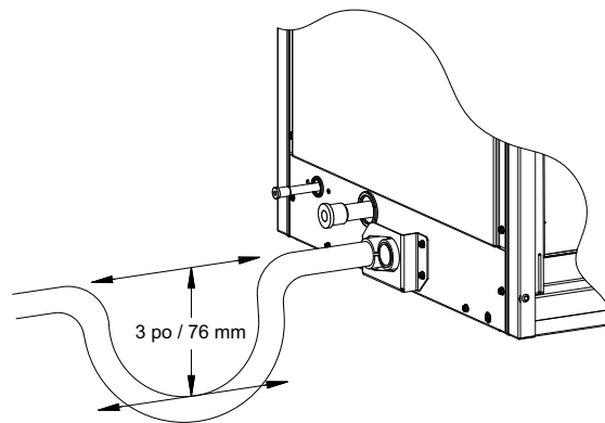
Figure 8 – Siphon de condensat
