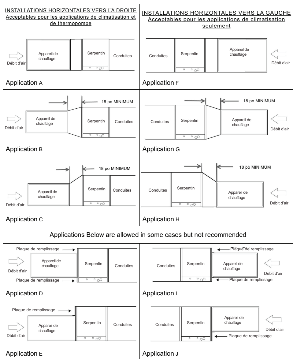
Figure 4 – Applications d'installation horizontale
