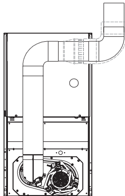
Upflow Application-Vent Elbow Up
