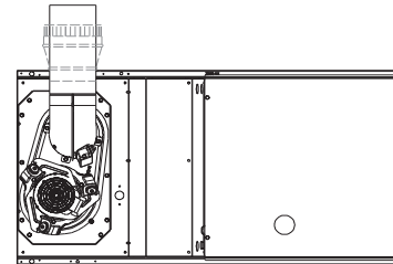
Horizontal Left Application-Vent Elbow Up
