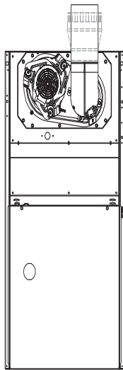
Upflow Application-Vent Elbow Up
