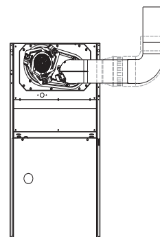
Upflow Application-Vent Elbow Right
