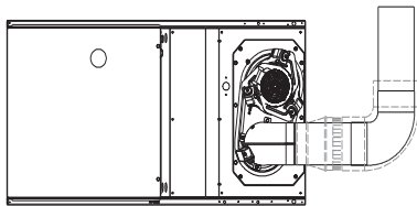
Horizontal Right Application-Vent Elbow Right
