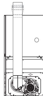
Horizontal Right Application-Vent Elbow Left
