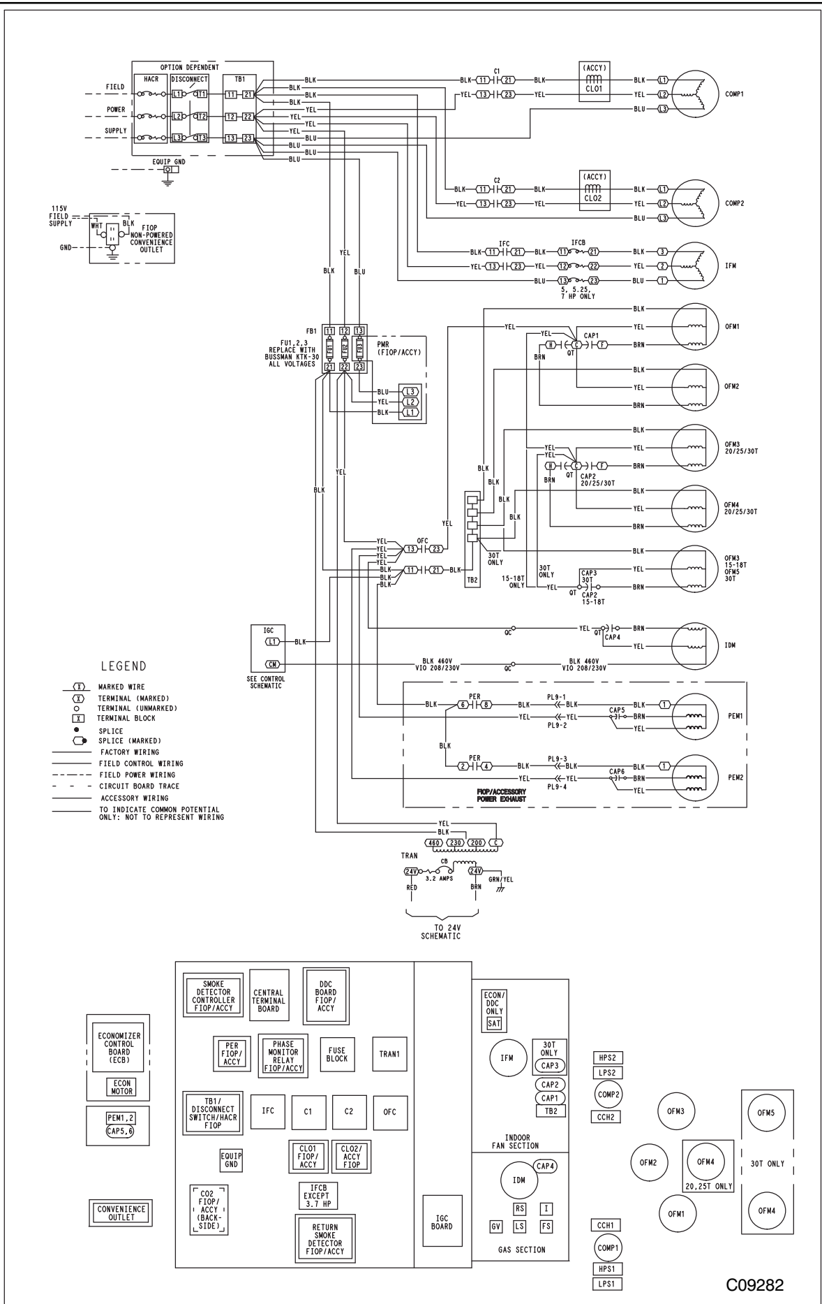
Fig. 4 Typical Power Diagram (All Voltages)
