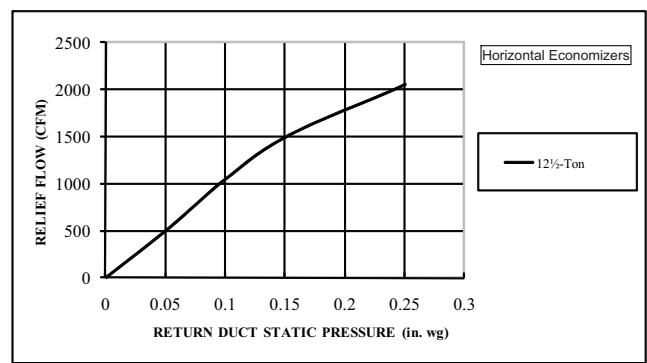
Fig. 23 – Barometric Relief Flow-Horizontal 12.5 Ton
