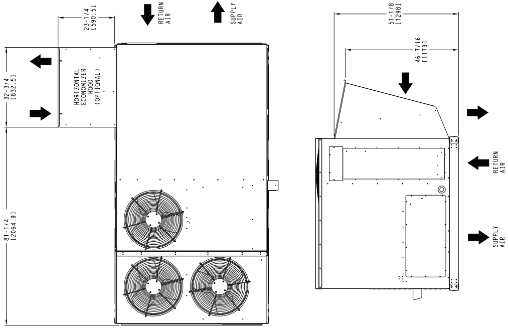
HORIZONTAL ECONOMIZER
