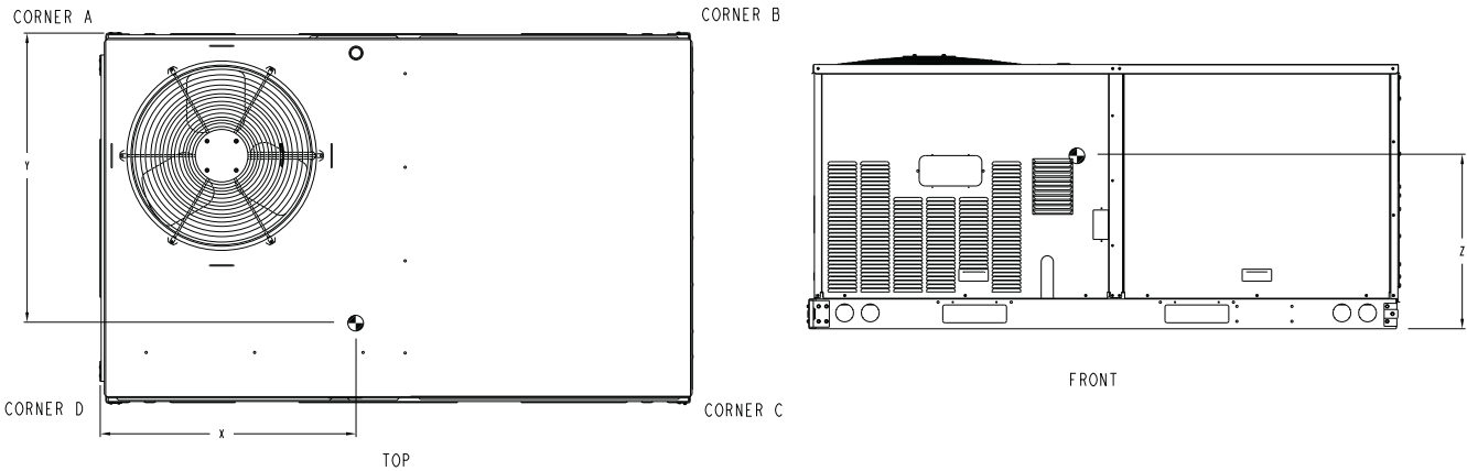
Fig. 2 – Dimensions RGH036–060
