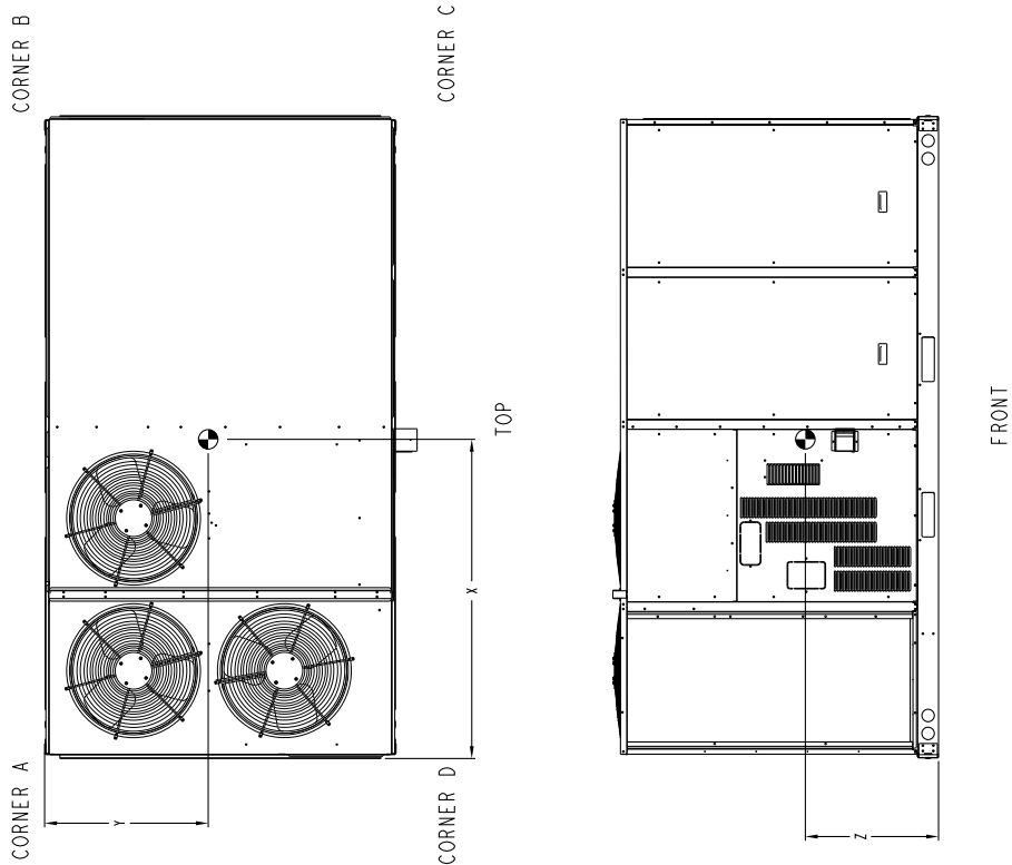
Fig. 13 - Dimensions RGH150
