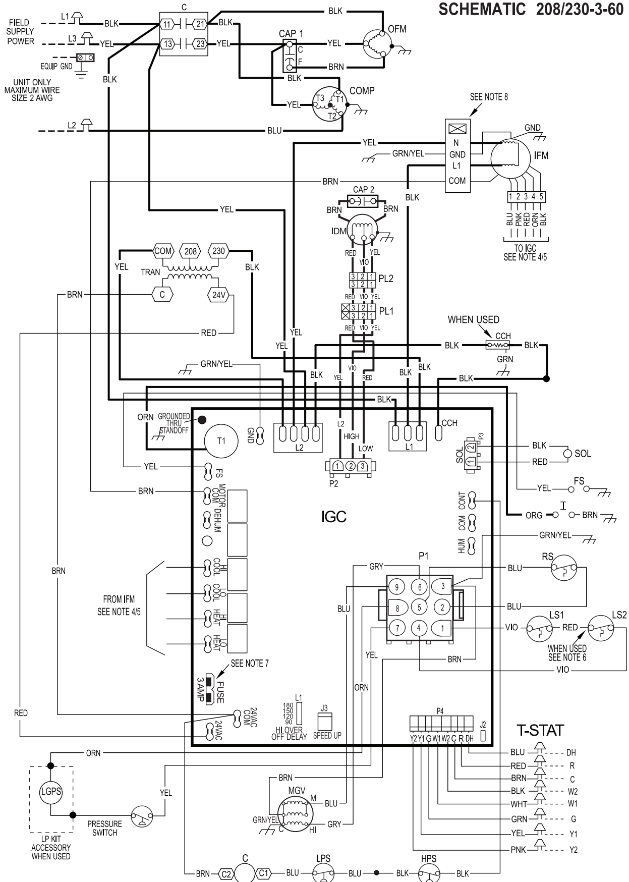
Fig. 15 - 208/230-3-60 Connection Wiring Diagram Gas Inputs 40, 60, 90 KBtu/hr
