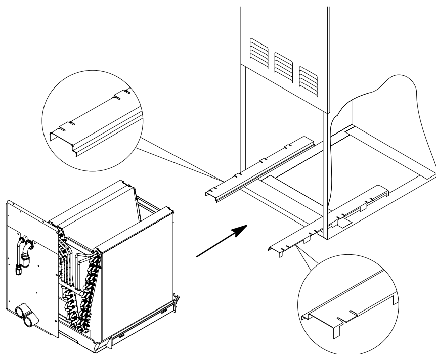
Figure 1 Longerons
