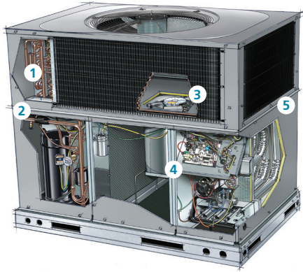
Standard Model
