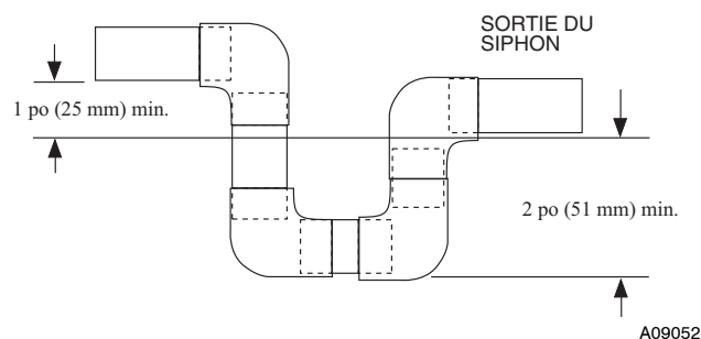
Figure 7 – Siphon de condensat
