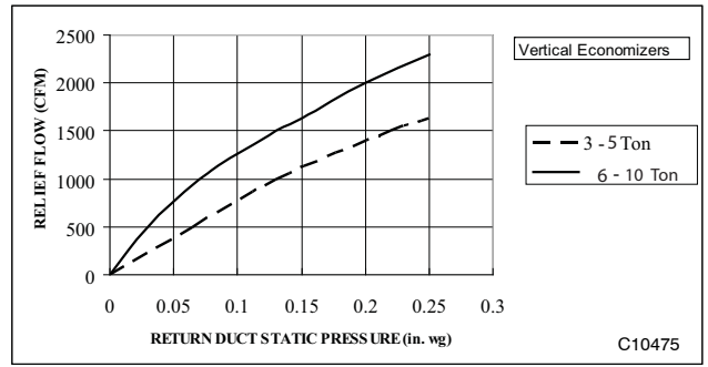
Fig. 6 Barometric Relief Flow – Vertical 3 – 10 Ton
